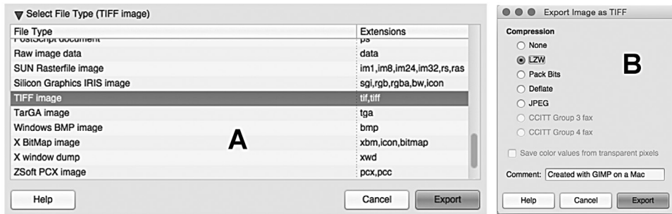
Figure 6. GNU Image Manipulation Program. A Portion of the “Export Image” window, showing the “Select File Type” menu with the settings for a TIFF image B “Export Image as TIFF” window, with the settings for LZW compression.
