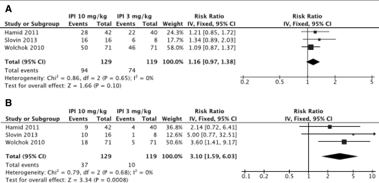
Fig. 4 Risk ratio of developing an irAE with ipilimumab at 10 mg/kg compared with 3 mg/kg for global irAEs all grade (a) and high grade (b)
