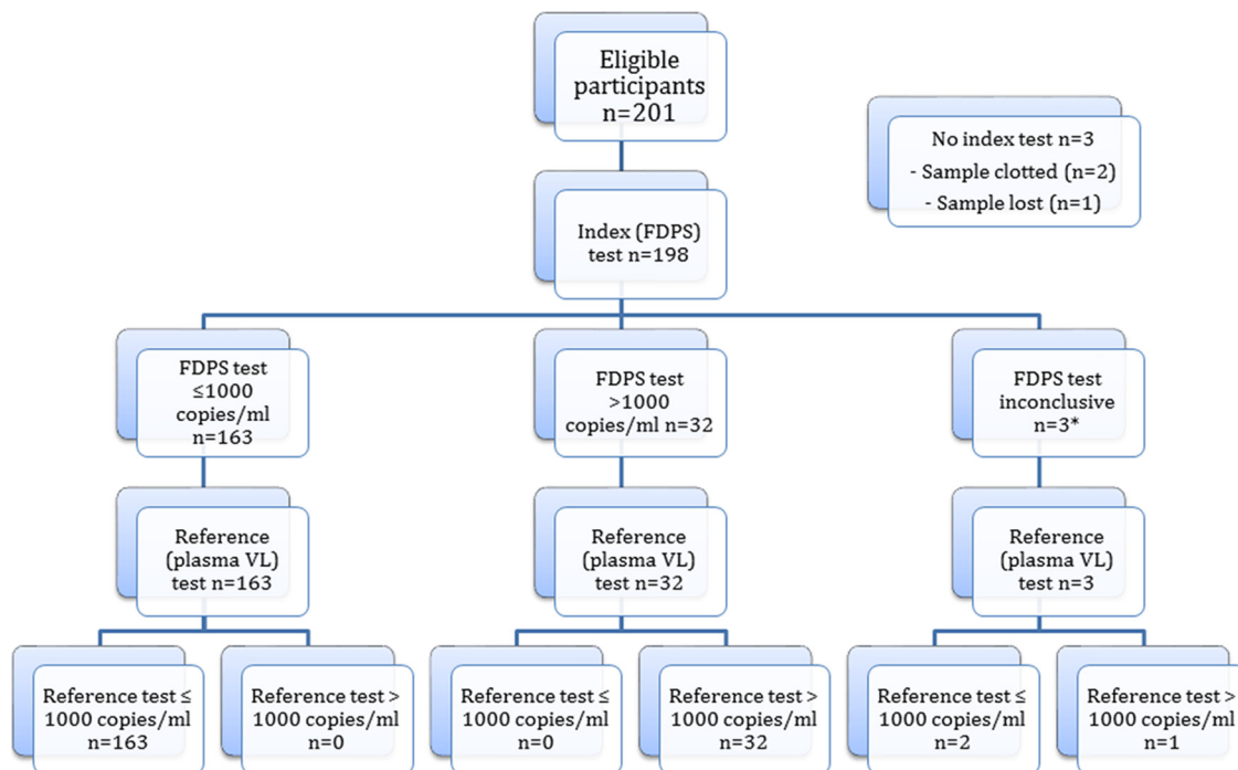
FIG 1 Flow diagram of FDPS VL test performance at a cutoff of 1,000 copies/ml according to STARD guidelines. The asterisk indicates that three FDPS samples failed to provide a valid viral load result on the Roche Cobas AmpliPrep/Cobas TaqMan platform.
