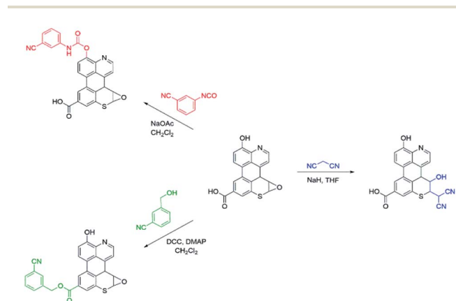
Scheme 1 Chemical tests that were used to quantify the functional groups displayed on sAO. The starting material shown in the centre represents a truncated form sAO and features pendant carboxylic acid, hydroxy, and epoxide groups. Using the reagents shown, the carboxylic acid groups were converted to esters, the hydroxyl groups were converted to carbamates, and epoxide groups were ring-opened. In all cases, the corresponding products feature nitrile groups (CN) that could be quantified using IR spectroscopy as well as elemental analysis.
