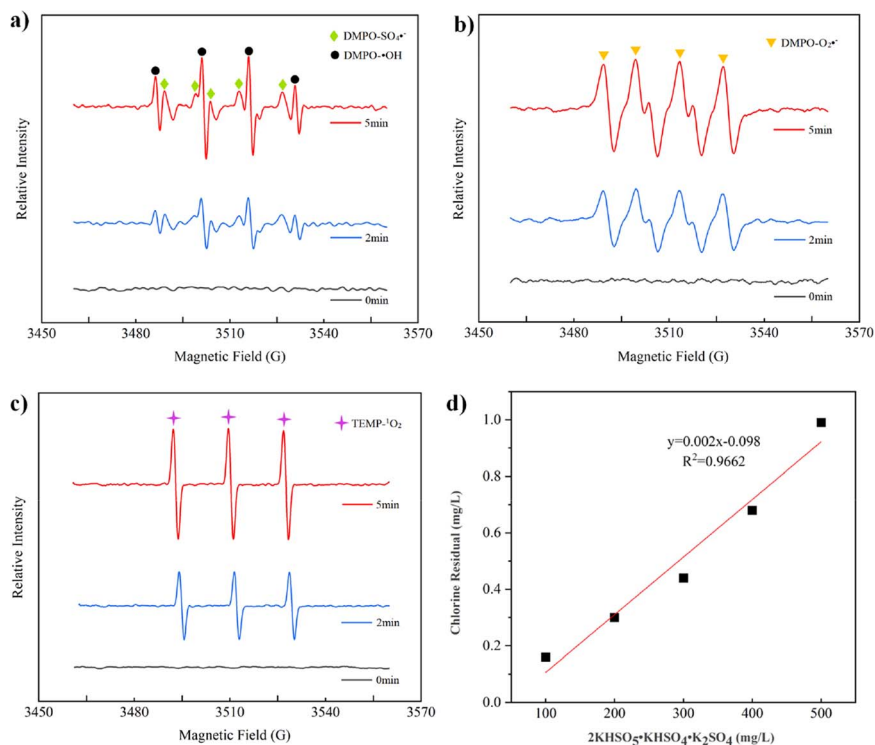
Fig. 3 (a) EPR detection mapping of HO * and SO 4 -* (DMPO capture); (b) EPR profiling of O 2 -* (DMPO capture). (c) EPR assays of 1 O 2 (TEMP capture). (d) Measurement of the residual chlorine concentration.
