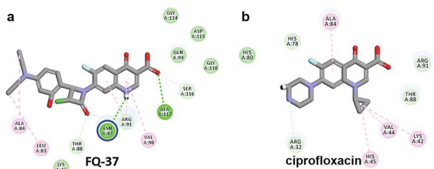
Fig. 8 (a) Hydrogen bond interaction of unsubstituted \text{-NH} group in molecule FQ-37 with mutant residue Asn87 (b) interactions of substituted \text{-NH} group in ciprofloxacin.
