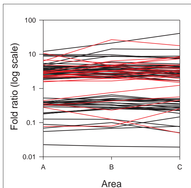
Figure 3 Transcript profiling of trees grown in area A, B, C and P.
