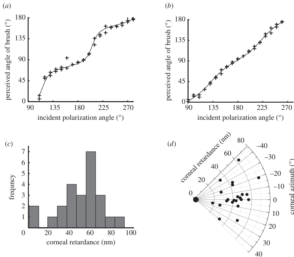
Figure 4. Nonlinear relationship between Haidinger's brushes (perceived polarization orientation) and the presented orientation of the polarized light field varied among individuals. In (a,b), each point is the reported orientation of the yellow axis of Haidinger's brushes relative to the orientation of the polarized stimulus produced by a modified LCD screen that was rotated around 180^\circ . The solid line is the nonlinear least-squares regression fit to equation (2.2) provided in the text. (a) The individual with the strongest nonlinearity in perceived angle as a function of stimulus polarization angle orientation. This individual had the highest estimated corneal retardance in our study, 71.4^\circ corresponding to 91.4 nm ( r^2 = 0.987 ). (b) An individual with an estimated retardance of 43.3^\circ , which corresponds to 55.3 nm at 460 nm ( r^2 = 0.997 ). This is similar to the mean retardance value found in the population tested and shows only a slight nonlinearity. (c) Histogram of the corneal retardance values for 24 participants. (d) Distribution of the corneal retardance and corneal azimuth values for all participants; larger point at origin represents two individuals with zero retardance.
