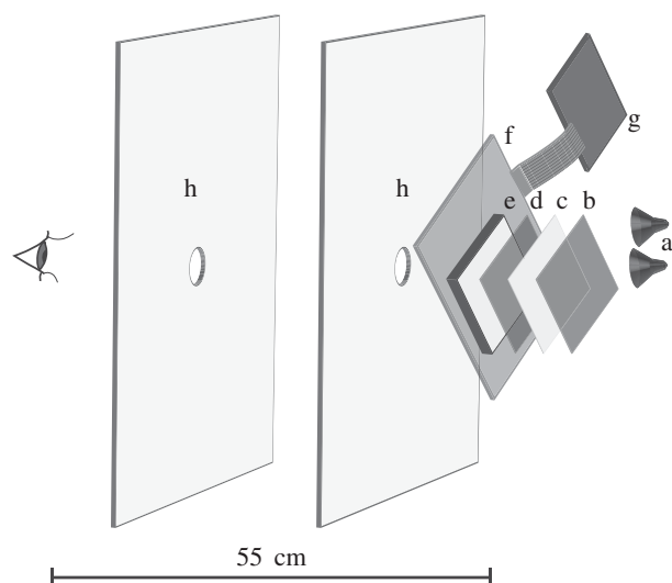
Figure 1. Schematic diagram of the modified LCD for presenting visual stimuli in polarization-only contrast at different per cent polarization levels. Light from two 6 W white LEDs (a) passed through a neutral density filter (b) if required (see supplementary table S1), and was then depolarized by a thin sheet of Teflon (c), before passing through a linear polarizer (d). It was then partially depolarized by one of our custom-made volume diffusers (e), after which the angle of polarization was rotated by a twisted nematic liquid crystal panel (f) from which the electronics (g) had been displaced. The various filters (b–e) were in close apposition in the actual device but are presented in an exploded format here to enable clear labelling and visualization. The image on the front of the modified LCD was positioned 55 cm from the eye of the observer and was only visible when viewed through two cardboard panels with aligned apertures (h), which limited the field of view to 5.9^\circ .
