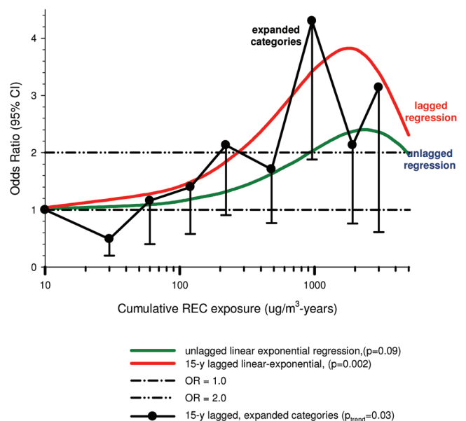
Figure 21. Odds ratios for lung cancer and cumulative REC in expanded category and linear-exponential ( \beta = 0.0043, \lambda = -0.00056 ) models lagged 15-years and unlagged linear-exponential ( \beta = 0.0016, \lambda = -0.00042 ) regression models from Tables S1, S2 and S3 in Silverman et al. (2012)
