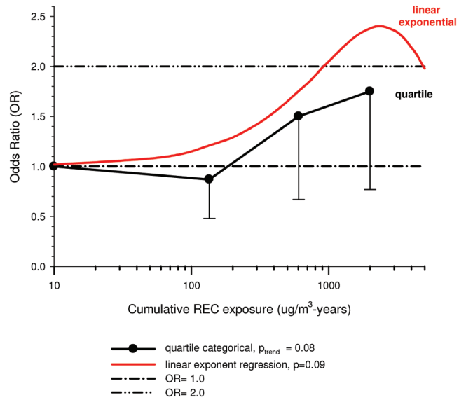
Figure 20. Odds ratios (ORs) and 95% confidence intervals for unlagged cumulative REC exposure and lung cancer in quartile and linear-exponential ( \beta = 0.0016, \lambda = -0.00042 ) regression models in DEMS nested case-control Tables 3 and S3 in Silverman et al. (2012).
