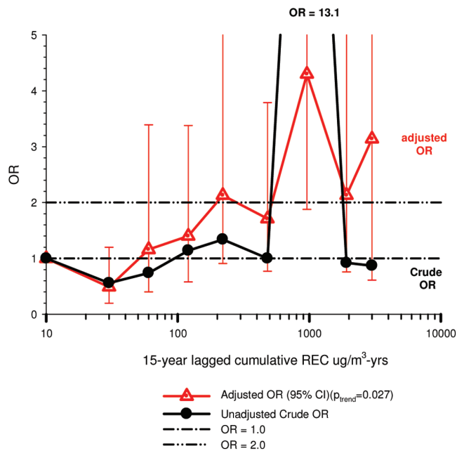
Figure 27. Crude and adjusted ORs for lung cancer and 15-years lagged cumulative REC for expanded exposure categories; ORs adjusted for smoking \times mine work location, >5 -year history of respiratory disease, and >10 -year history of high risk jobs for lung cancer; crude ORs calculated from Table S2 in Silverman et al. (2012).
