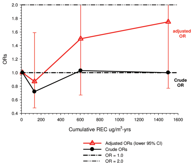
Figure 25. Crude and adjusted ORs for lung cancer and unlagged cumulative REC; ORs adjusted for 24 smoking \times mine location, history of respiratory disease >5 -years and history of high risk job for lung cancer >10 -years; Crude ORs calculated from Table 3 in Silverman et al., 2012.
