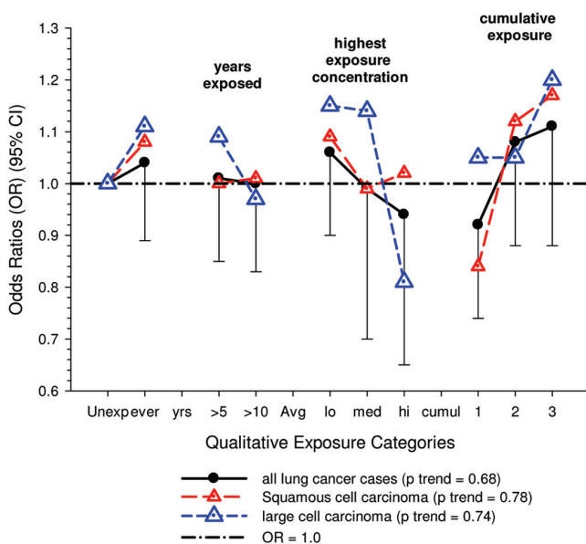
Figure 5. Adjusted odds ratios of lung cancer in relation to occupational exposures to gasoline emissions, men 40+ from Canadian hospital-based case-control study; ORs adjusted for age, province, pack-years, second-hand smoke, silica (Y/N) and asbestos (Y/N) ( p values refer to cumulative exposure) (Villeneuve et al., 2011).
