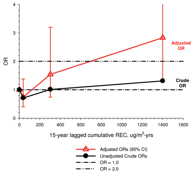
Figure 26. Crude and adjusted ORs for lung cancer and 15-year lagged cumulative REC; ORs adjusted for smoking \times mine location interaction; >5 -year history of respiratory disease and >10 -year history of high risk jobs for lung cancer; crude ORs calculated from Table 3 in Silverman et al. (2012).
