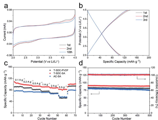
Fig. 6 Electrochemical performances of the T-SDC and AC in half-cells with a potential window of 2.0–4.5 V. (a) CV curves of the T-SDC-SA electrode for the 1 st , 2 nd and 10 th cycles at a scan rate of 0.2 mV s -1 , (b) GCD curves of T-SDC-SA at 0.1 A g -1 , (c) rate performance and (d) cycling performance for 500 cycles at a current density of 1 A g -1 .
