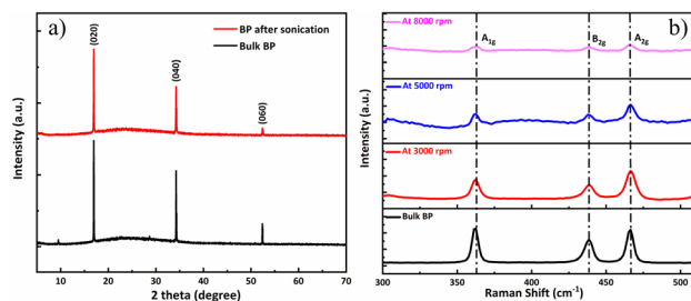
Fig. 4 (a) Comparison of XRD patterns of bulk BP and fabricated BP supernatant after the sonication process. (b) Comparison of the Raman spectra between bulk BP crystals and fabricated BP dispersions after the centrifugation process (3000, 5000, and 8000 rpm, respectively).
