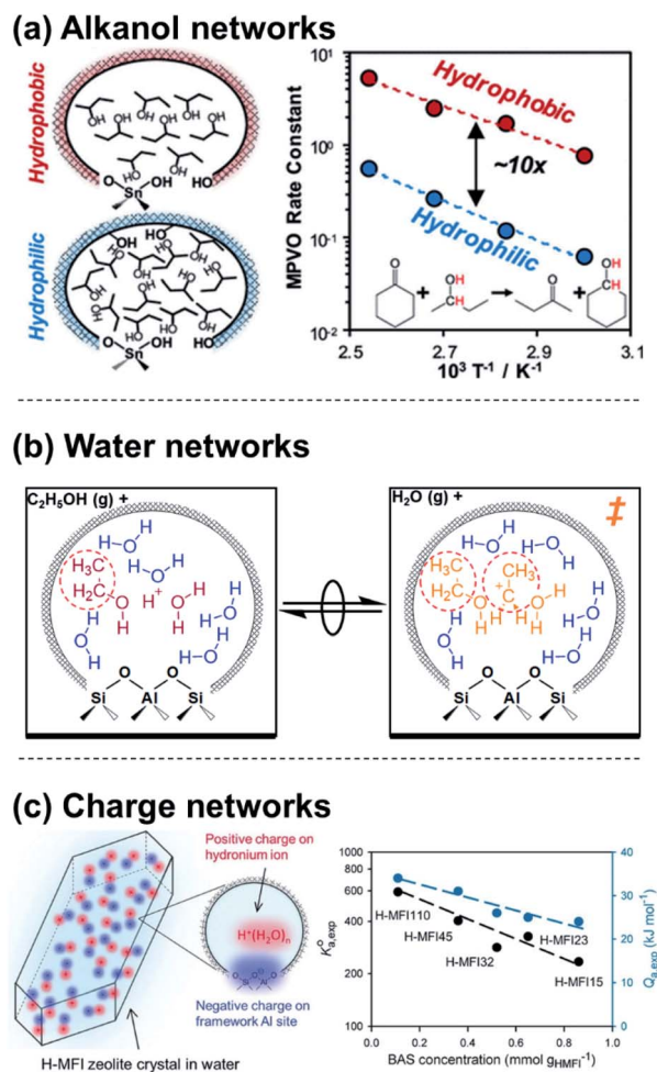
Fig. 3 Examples of (a) extended alkanol networks within non-polar Sn- \beta zeolites, 76 (b) extended H_2O networks within Brønsted acid zeolites, 53 and (c) adsorption properties that depend on networks of charge and their density within Brønsted acid zeolites. 17 (a) Adapted from ref. 76 with permission from the American Chemical Society, copyright 2020. (b) Adapted from ref. 53 with permission from the Royal Society of Chemistry, copyright 2020. (c) Adapted from ref. 17 with permission from John Wiley and Sons, copyright 2019.
