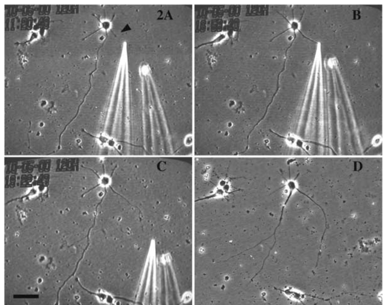
Figure 2. Elongation of a minor process of a stage 3 neuron induced by experimentally applied tension.
