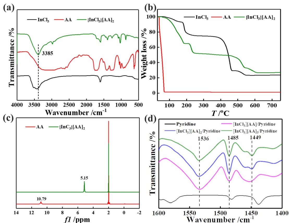
Fig. 1 (a) FT-IR spectra of InCl 3 , AA and [InCl 3 ][AA] 2 . (b) TG spectra of InCl 3 , AA and [InCl 3 ][AA] 2 . (c) 1 H NMR spectra of AA and [InCl 3 ][AA] 2 in DMSO. (d) FT-IR spectra were obtained using pyridine as the probe molecule, with a volume ratio of DES to pyridine being 1 : 2.
