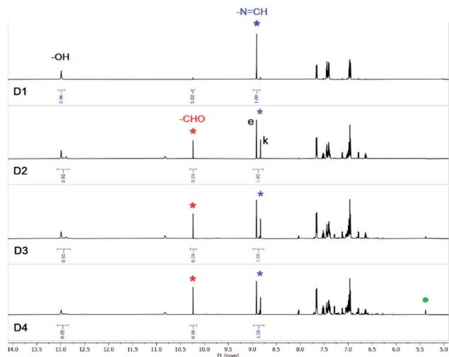
Fig. 7 Aromatic region of ^1\text{H-NMR} spectra ( \text{DMSO-d}_6 ) of CL2 in the presence of 15 equivalents of \text{H}_2\text{O} , recorded after 1 hour (D1), 24 hours (D2), 48 hours (D3) and after 72 hours (D4). Signals labelled with e and k indicate the enol and keto forms of CL2 respectively. Signals labelled with red and blue asterisk indicate -\text{CHO} and -\text{N}=\text{CH}- peaks of salicylaldehyde (red) and CL2 (blue) respectively.
