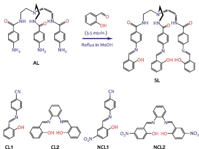
Scheme 1 Molecular structures of salicylidene Schiff bases studied here (synthesis details are provided in the ESI†).
