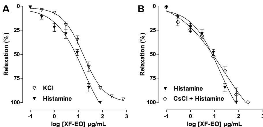
Fig. 3 Effect of XF-EO on tonic contractions induced by KCl (40 mM) (▽) or histamine ( 10^{-6} M) in both absence (▼) (a) and presence (◇) of CsCl (5 mM) (b) on guinea pig ileum ( n = 3-5 ). Symbols and vertical bars represent mean and S.E.M., respectively
