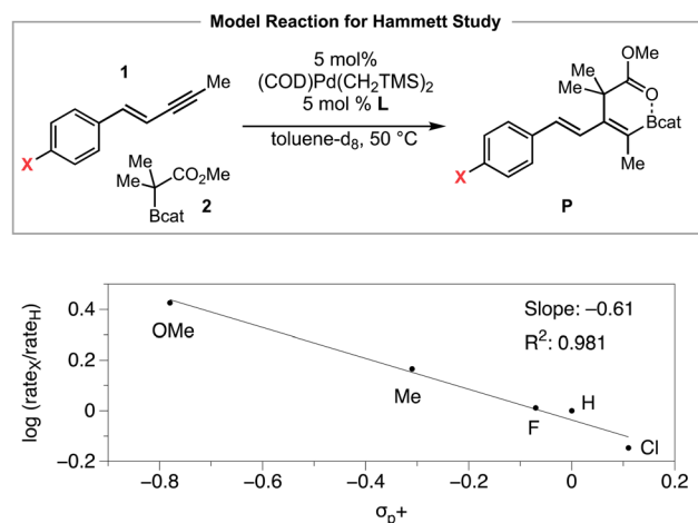
Scheme 5 Hammett analysis.
