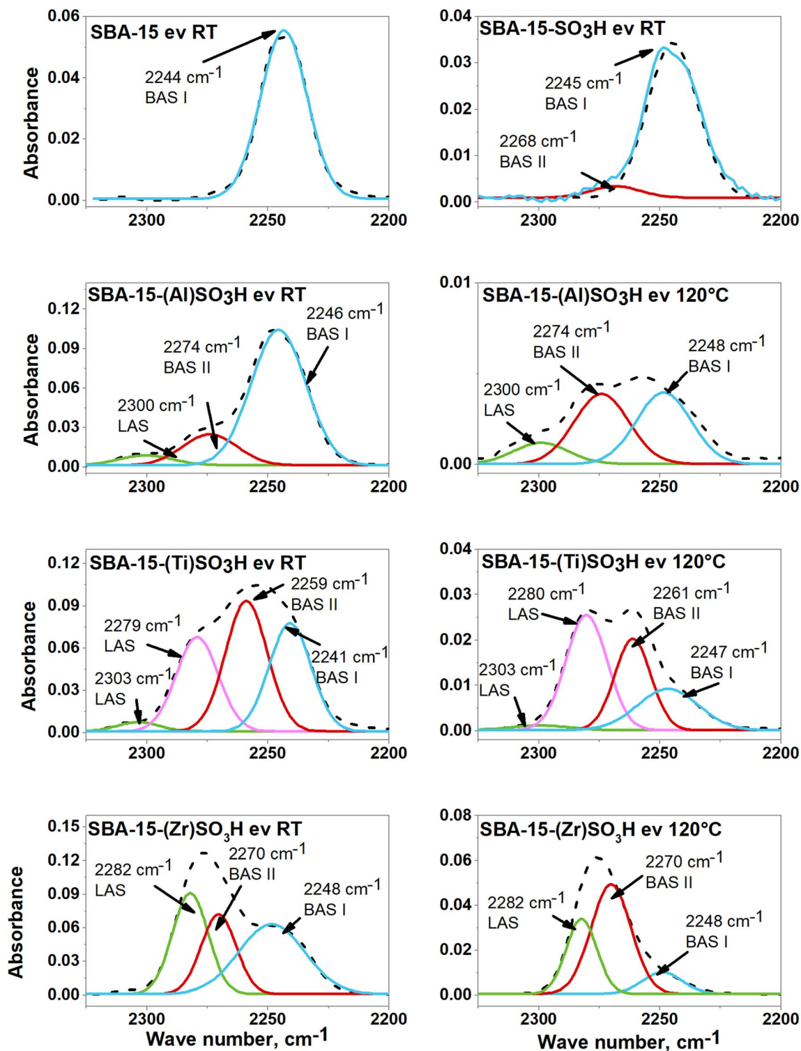
Fig. 5 FTIR spectra of SBA-15-(X) \text{SO}_3\text{H} with adsorbed pivalonitrile outgassed at room temperature (ev RT) and 120 °C (ev 120 °C). LAS: Lewis acid site, BAS I: Brønsted acid site type I, BAS II: Brønsted acid site type II, - - - original spectra.
