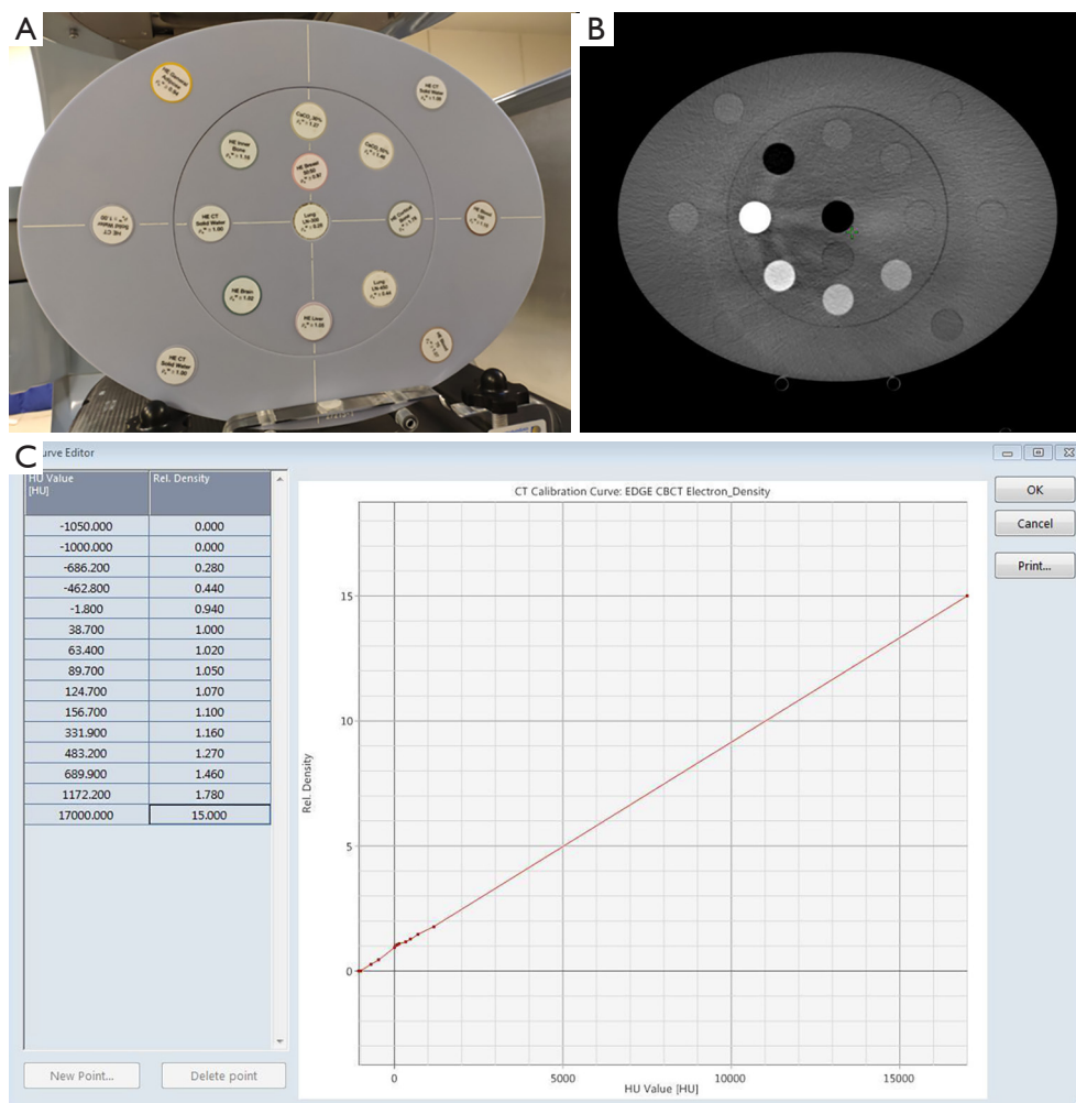
Figure 1 Hounsfield units to electron density calibration. (A) Advanced Electron Density Phantom Model 1467. (B) CBCT image for the phantom. (C) The calibration curve of HUs to ED. CBCT, cone-beam computed tomography; HUs, Hounsfield units; ED, electron density.
