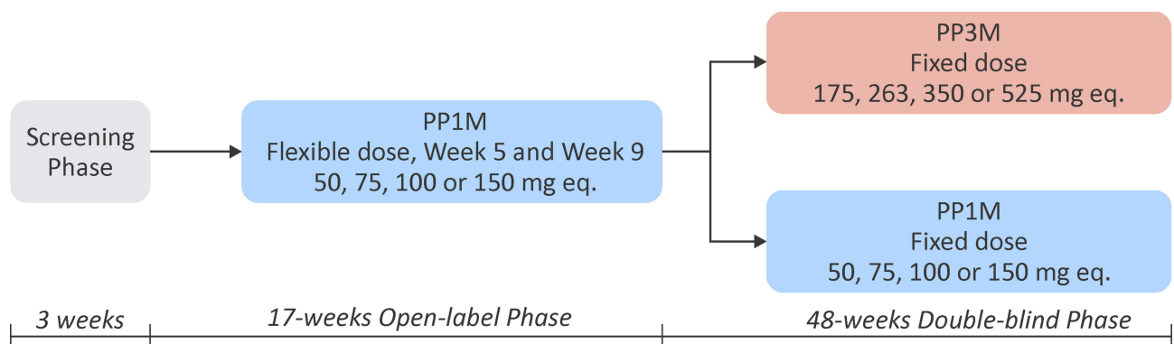
Figure 1 Study profile.
