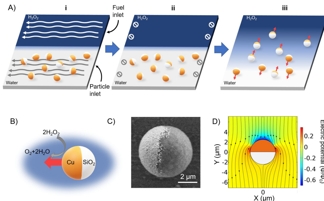
Figure 2. Intrinsic propulsion and chemotaxis of \text{Cu}@/\text{SiO}_2 micromotors. A) Operating principles of the positive and negative chemotaxis of \text{Cu}@/\text{SiO}_2 micromotors. B) Schematic diagram of the intrinsic propulsion of \text{Cu}@/\text{SiO}_2 micromotors in \text{H}_2\text{O}_2 . C) Scanning electrical micrograph of a \text{Cu}@/\text{SiO}_2 microsphere. D) Electric potential (color coded) and flow field lines (black arrows) around a \text{Cu}@/\text{SiO}_2 Janus micromotors.
