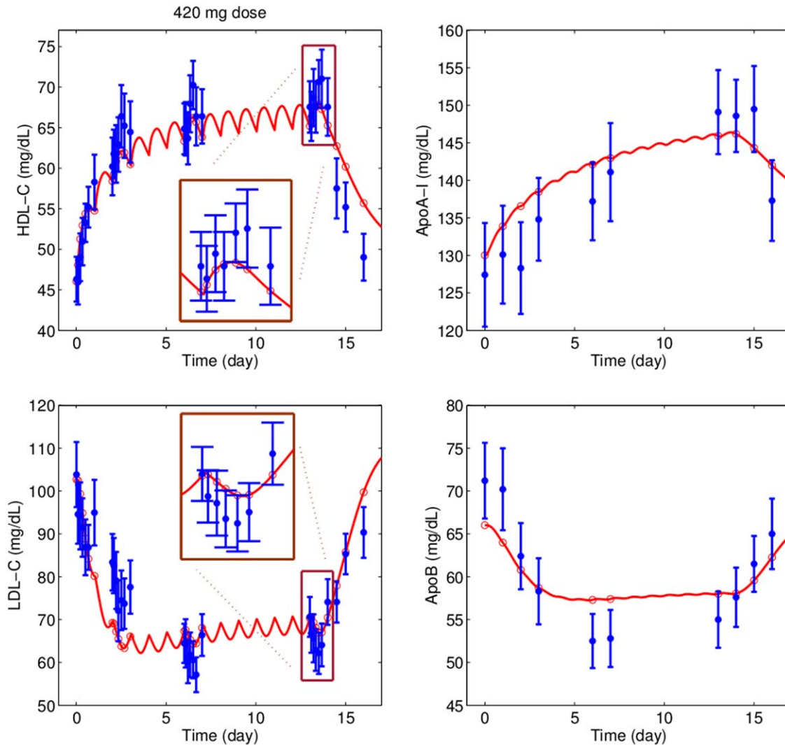
Figure 3 Fit of the systems pharmacology model simulation to the MAD data (mean±SEM) for the 420 mg dose group.
