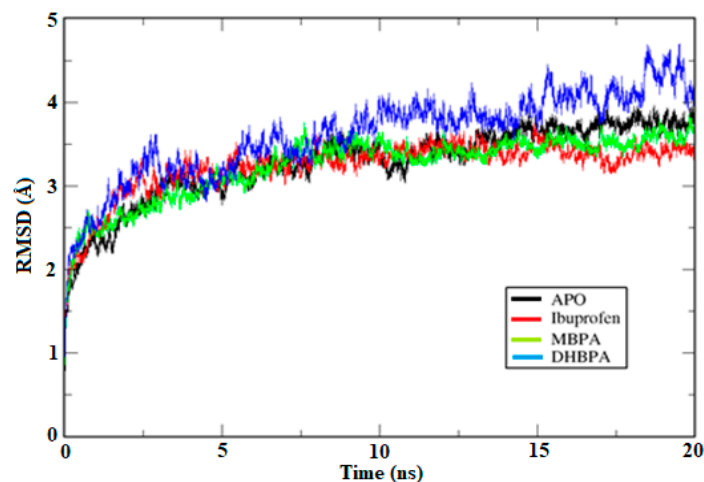
Figure 4. Root-mean-square deviation of atomic positions (RMSD) graph of COX-2 with compounds plotted in the XMGrace program.
