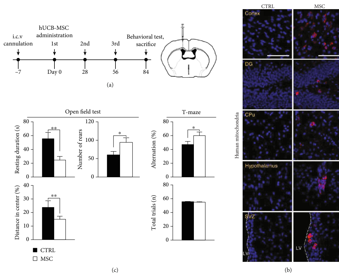
FIGURE 1: Administration of hUCB-MSCs ameliorates behavioral dysfunction in 5xFAD mice. (a) The schedule of repeated injection (3 times) of hUCB-MSCs via the lateral ventricle of 5xFAD mice, which express human APP and PSEN1 transgenes with a total of five AD-linked mutations. After 4 weeks at the last injection, mice were subjected to behavioral tests, and the brains were collected to analyze tau phosphorylation with western blotting or IF. (b) The brains injected with hUCB-MSCs were stained with antihuman mitochondria (red). Fluorescence signals were observed in the cortex, DG, CPu, hypothalamus, and SVZ (scale bar = 100 μm). (c) Various behavioral tests for hUCB-MSCs-injected 5xFAD mice (open field: resting duration, the distance in center, and number of rears; T-maze: alternation; n = 8 per group; * p < 0.05 , ** p < 0.005 ). CTRL: PBS-administrated 5xFAD; MSC: hUCB-MSC-administered 5xFAD.
