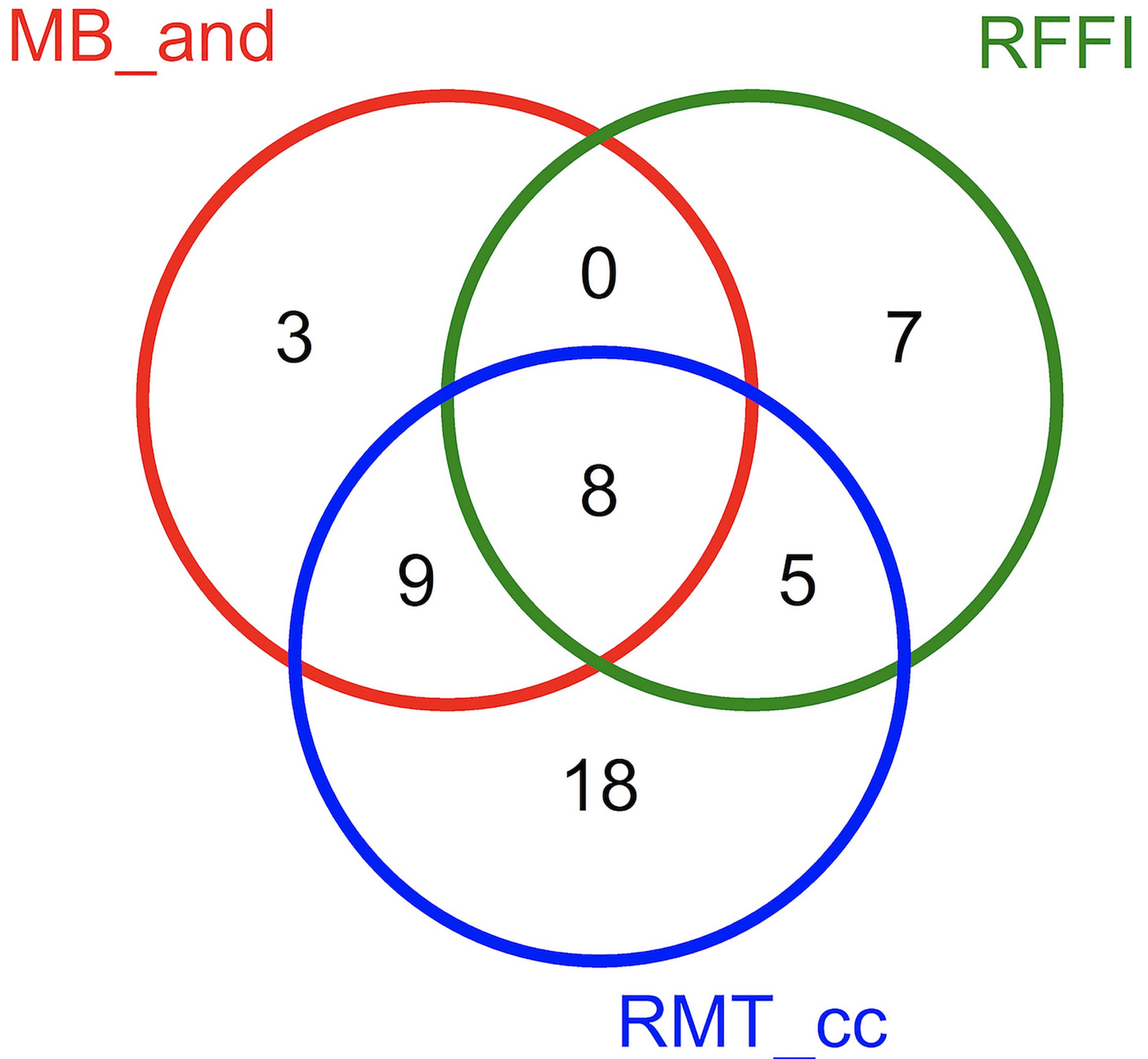
Fig 2. Venn diagram of unique and shared features selected using RF Feature Importance (RFFI), network-based feature selection applied to MB (RMT) networks and using 'and' ('cc') for node importance scoring.
