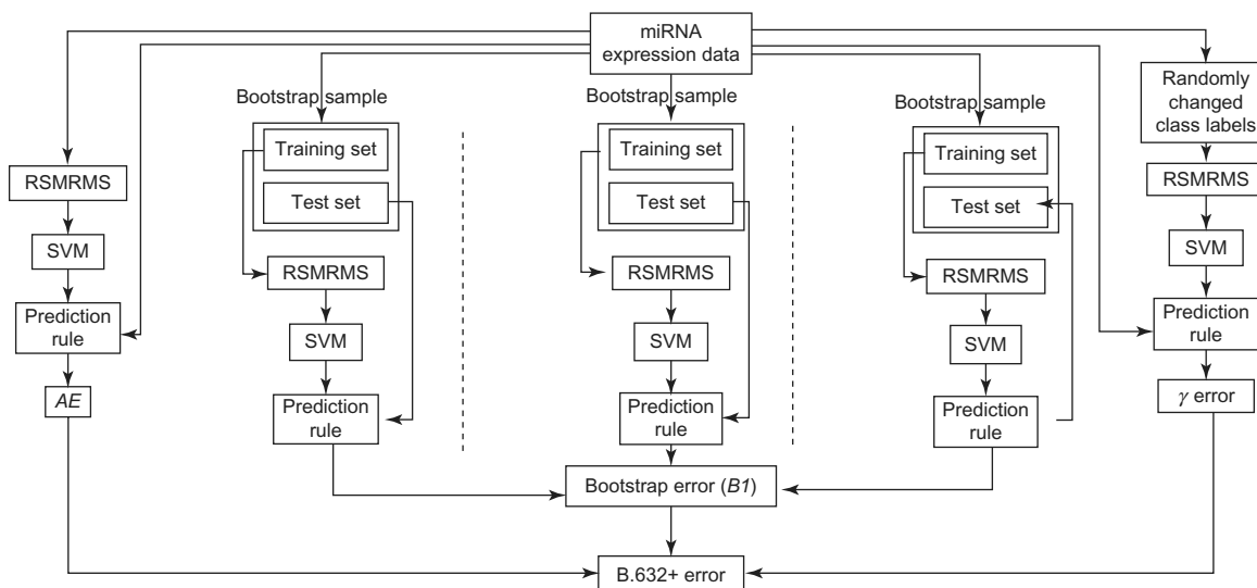
Figure 1 Schematic flow diagram of the proposed in silico approach for identification of differentially expressed miRNAs. Abbreviations: miRNA, microRNA; RSMRMS, rough set-based maximum relevance maximum significance criterion; SVM, support vector machine; AE, apparent error; \gamma error, no-information error.
