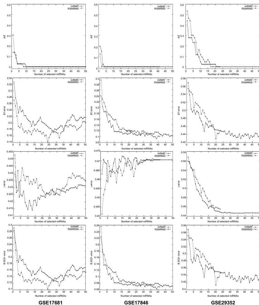
Figure 5 Error rates of the SVM obtained using the mRMR and RSMRMS algorithms averaged over 50 random splits. Abbreviations: SVM, support vector machine; mRMR, mutual information–based minimum redundancy–maximum relevance; RSMRMS, rough set–based maximum relevance maximum significance; miRNA, microRNA; AE, apparent error; BI, bootstrap error; \gamma , no-information error; B.632+, B.632+ error.
