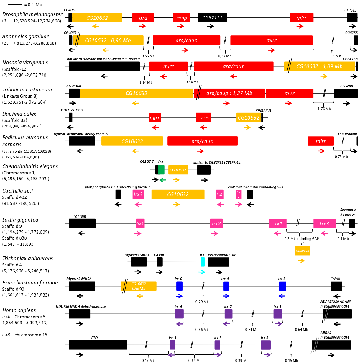
Figure 6 Genomic organization of selected lrx genes. The portion of the genome that includes the lrx gene(s) in several species is schematically depicted. The name of the genes that flank the lrx genes are those indicated in the genome browsers of the different species. In the case of Lottia , there is a gap in the genomic scaffold between lrx1 and lrx3 , and this region may include the CG10632 gene.
