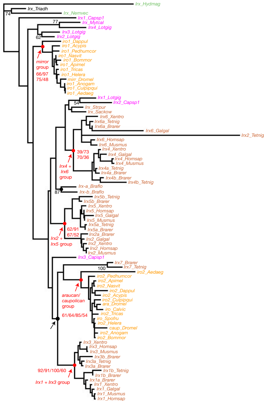
Figure 3 Phylogenetic analysis of Irx genes in metazoans. The represented tree is a maximum-likelihood tree, which has been rooted using the Irx gene from Hydra as outgroup (this should be considered as arbitrary rooting). This tree is based on a multiple alignment that includes the Irx conserved domains. The most important monophyletic groups are indicated in red and the associated numbers are their statistical support values obtained with different methods of phylogenetic reconstruction, as described in Figure 2. Statistical support in the maximum-likelihood analysis for some other internal branches is indicated in black. Only statistical support values >50% are shown except for a few cases. Other internal branches (with statistical support <50%) should be considered unreliable. The black arrow points to the group which is discussed in the main text.
