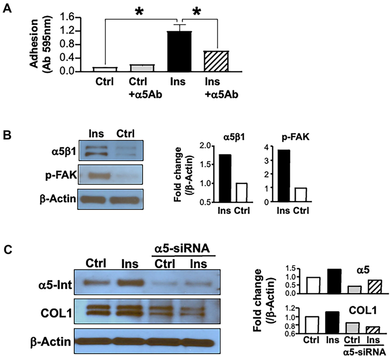
Figure 6. Insulin stimulates \alpha 5 \beta 1 integrin and its signaling pathway.
