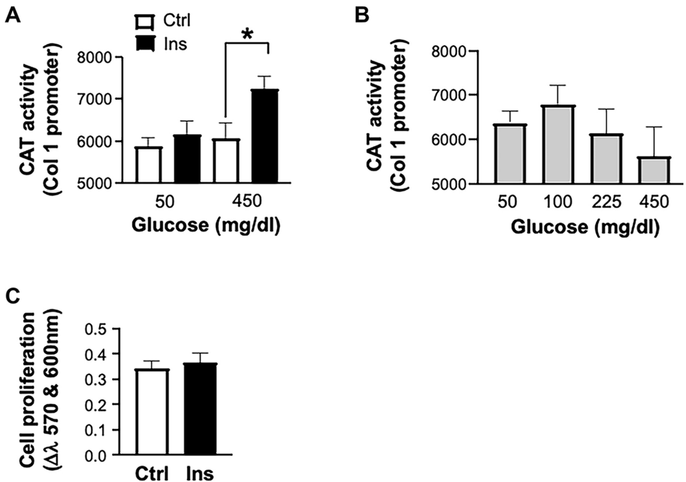
Figure 3. The effect of glucose and insulin on type I collagen synthesis and HSCs proliferation. Primary HSC cultures were incubated in DMEM enriched with 50 or 450 mg/dL glucose with (Ins, 5 \mu mol) or without (Ctrl) Ins. COL1 promoter activity was assayed as in the legend in Figure 2A (A). Promoter activity of COL1 was assayed in cells incubated with different glucose concentrations (in mg/dL, X-axis) without concomitant Ins treatment (B). Alamar blue assay was used to test the effect of Ins on cell proliferation. Cell proliferation was determined by a colorimetric change in the medium measured as a difference in culture media absorbance at 570 and 600 nm (C). HSCs: Hepatic stellate cells; DMEM: Dulbecco's modified Eagle Medium; COL1: type I collagen; Ins: insulin; Ctrl: control.
