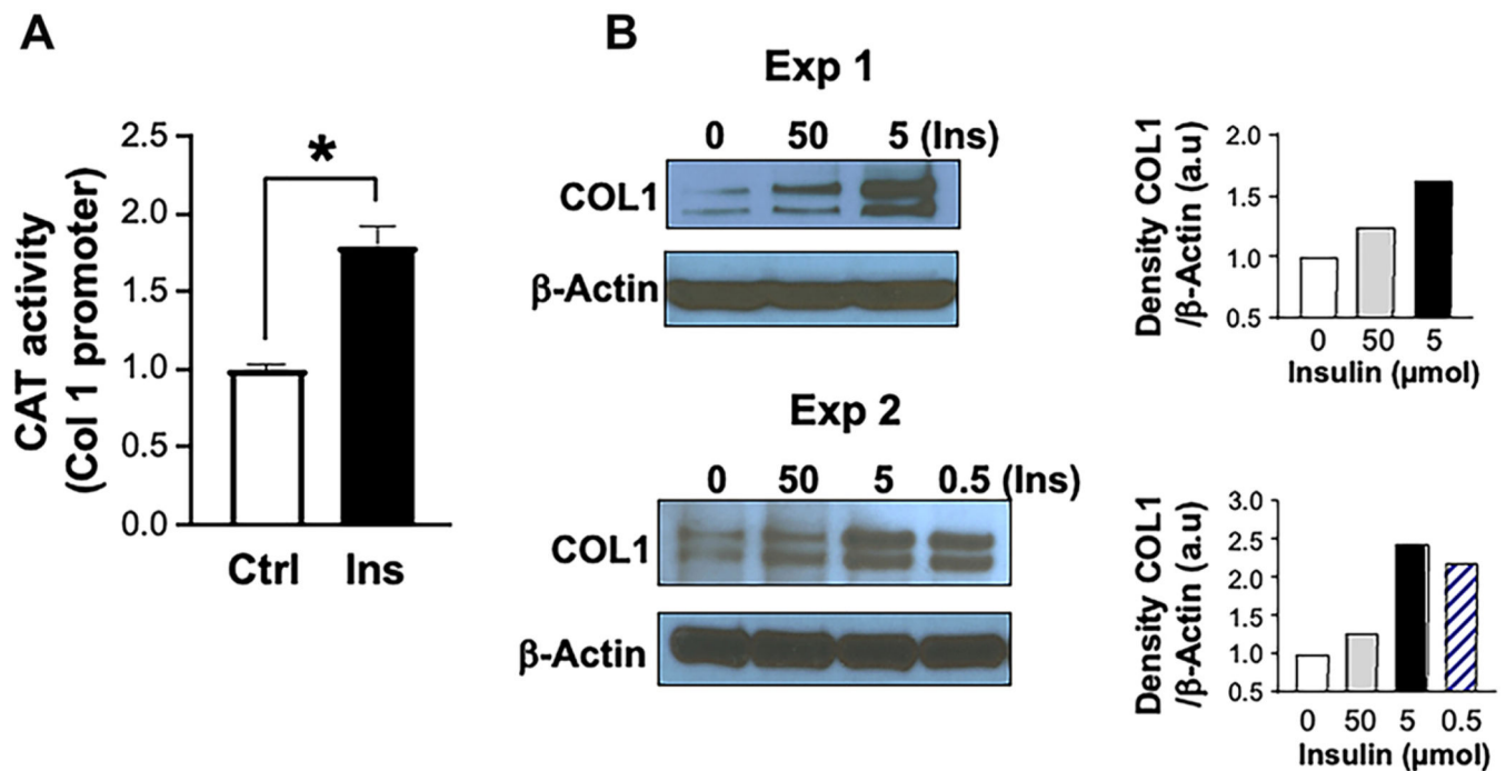
Figure 2. The insulin effect on type 1 collagen production.
