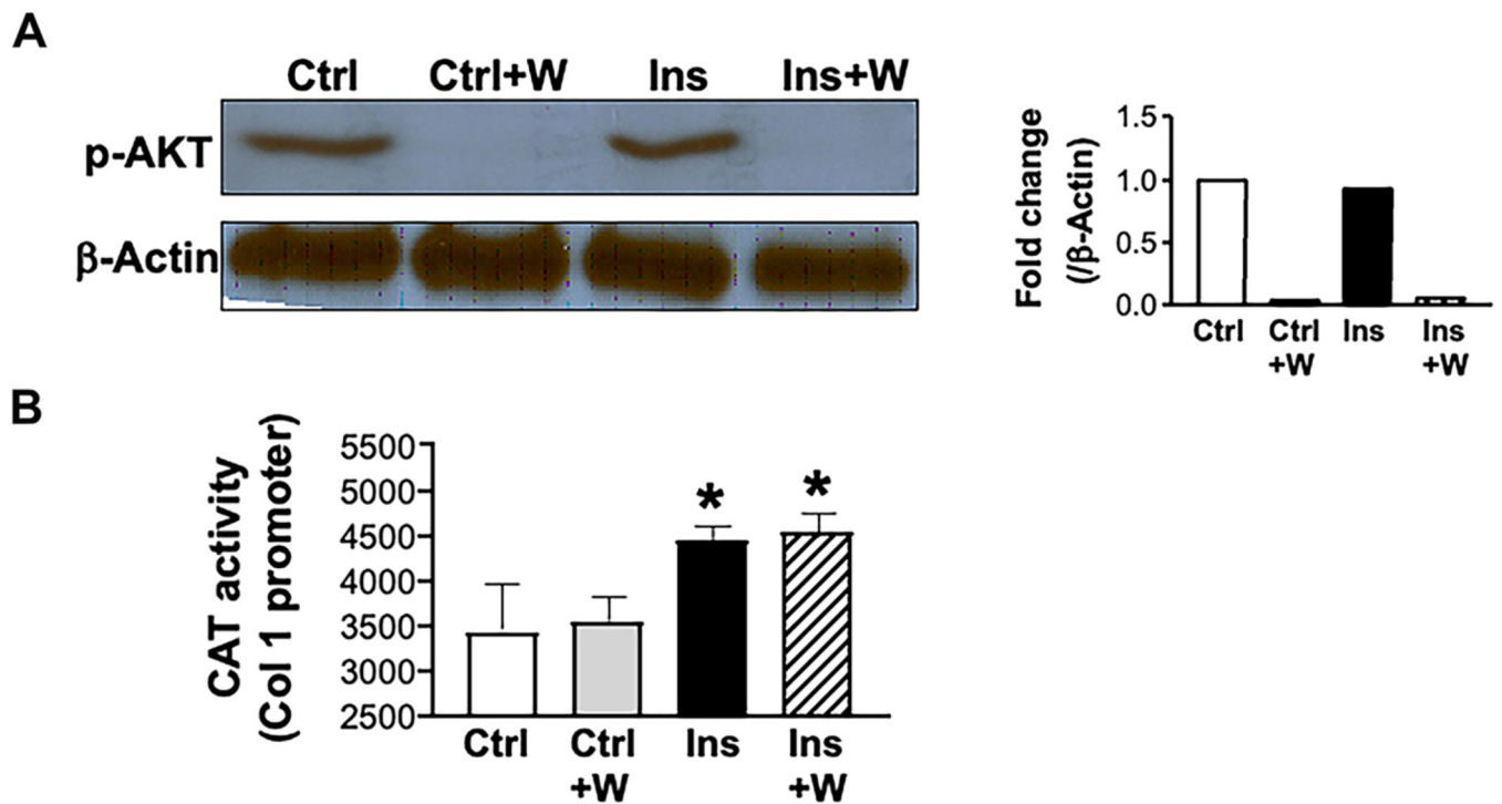
Figure 5. Insulin-induced collagen synthesis by HSCs is not mediated by the PI3 Kinase signaling pathway.
