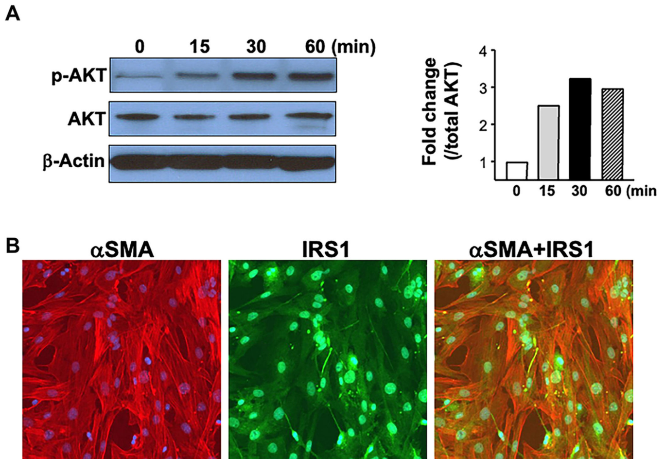
Figure 4. Insulin signaling in primary HSCs.
