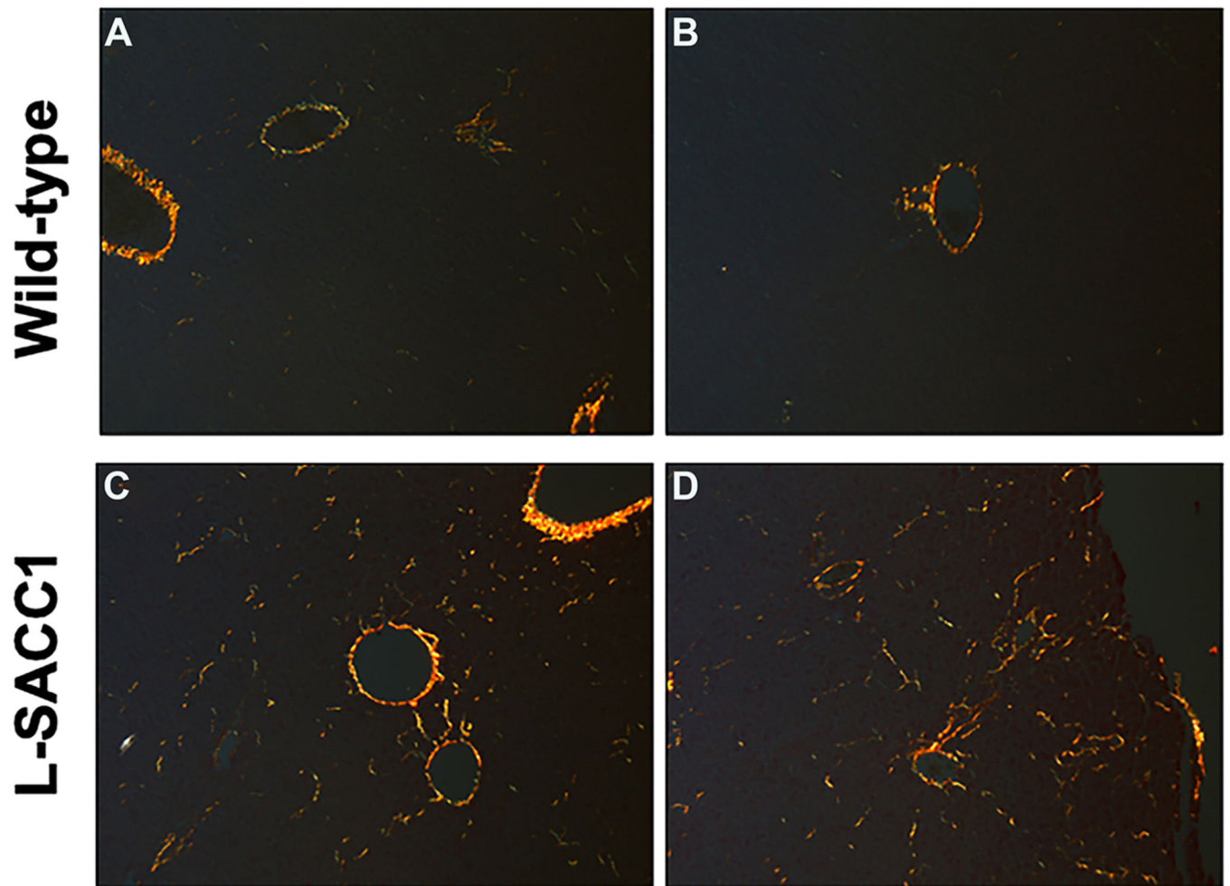
Figure 7. Type 1 collagen expression is increased in the livers of L-SACC1 transgenic mice. Sirius red staining (visualized under polarized light) of representative liver sections from wild-type (A and B) and L-SACC1 mice (C and D). L-SACC1 livers contain more stained birefringent COL1 fibers (seen as yellow on the black background). COL1: type I collagen.
