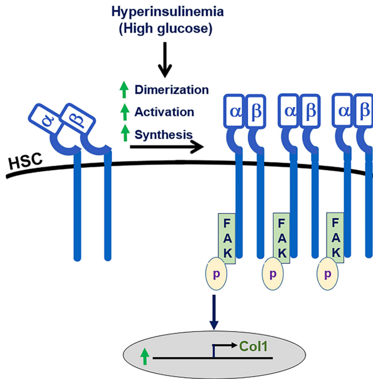
Figure 9. Proposed model of the effect of hyperinsulinemia and hyperglycemia on \alpha_5\beta_1 integrin signaling and type I collagen synthesis.
