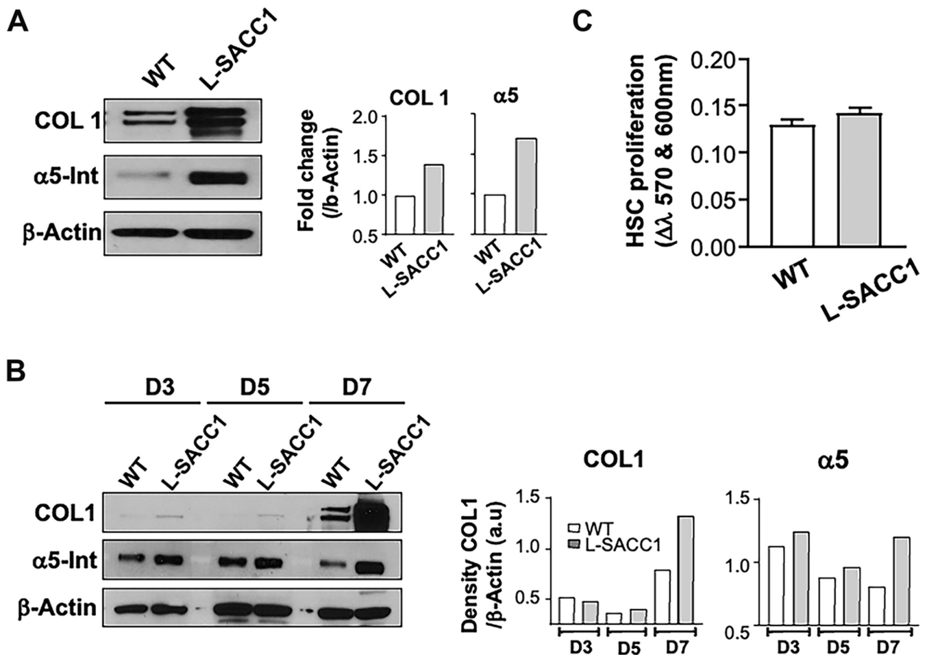
Figure 8. Elevated Type I collagen and α5β1 integrin levels in primary HSCs isolated from L-SACC1 mice.
