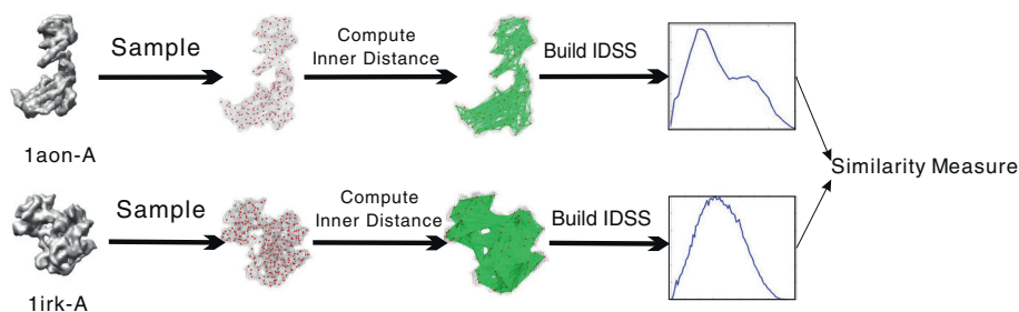
Figure 1 The illustration of flexible molecular shape comparison and similarity measure based on the IDSS histograms. Given a molecular shape, the whole process could be divided into three independent steps including sampling (red points) on the molecule, computing inner distances (green line segments) between all sample point pairs, and building the IDSS histogram. Consequently, our approach reduces the similarity measure among molecules to the comparison of IDSS histograms. An example is given for calculating the similarity measure between two different molecules (PDB codes: 1aon-A, 1irk-A), where the similarity score is equal to 0.6535.
