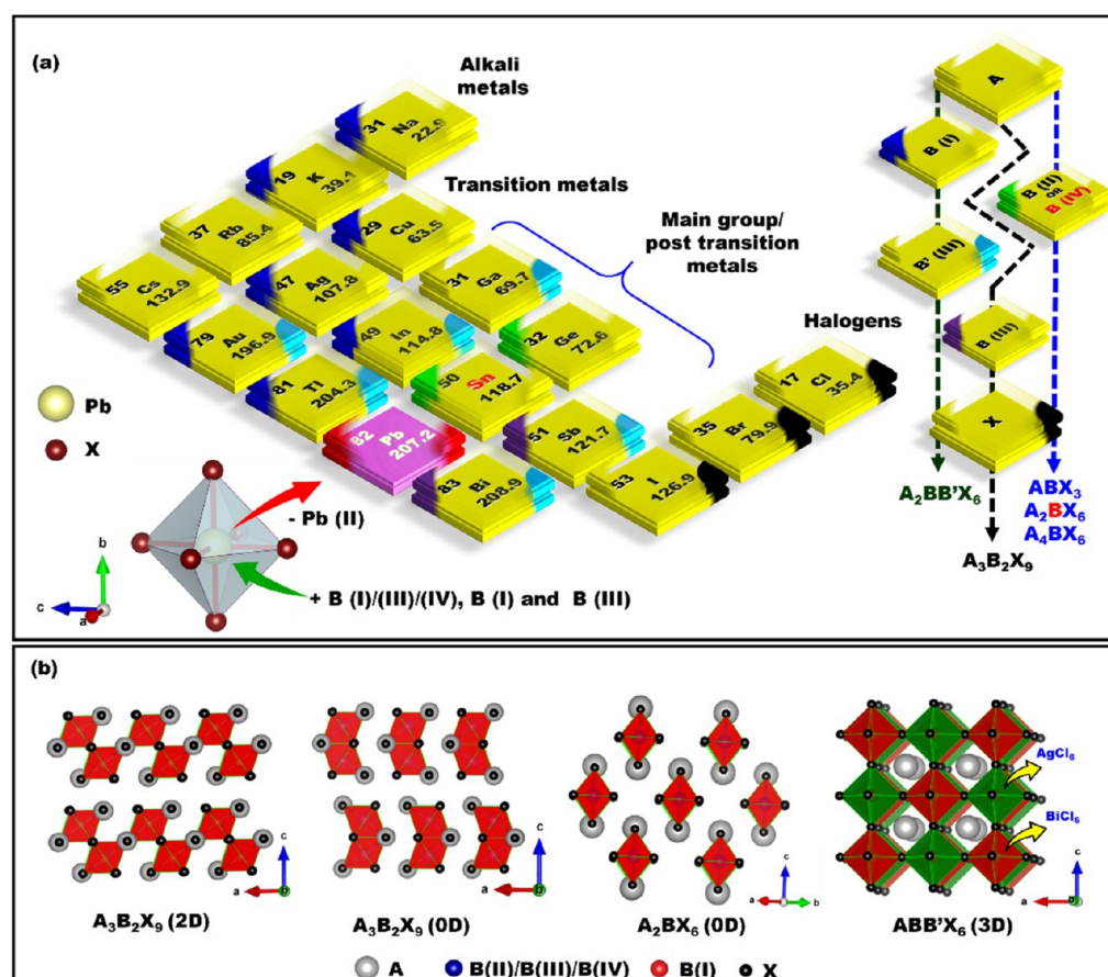
Figure 50. (a) Combinations of elements from a part of periodic table forming possible Pb-free metal-halide perovskite and their derivative structures. The triangular color code specifies the site occupancy as per the compositional formula presented in the extreme right. (b) Structural presentation of Pb-free metal-halide perovskites and perovskite derivatives showing network of octahedra in 3D, 2D, and 0D directions.
