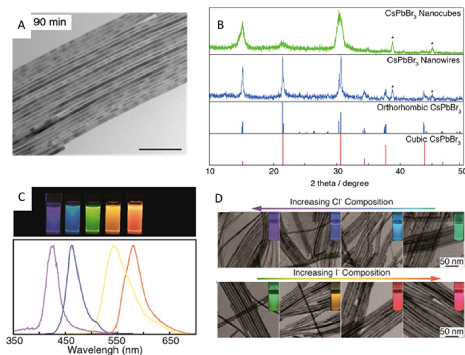
Figure 16. (A) TEM image of colloiddally synthesized \text{CsPbBr}_3 nanowires. (B) X-ray diffraction spectrum of \text{CsPbBr}_3 nanocubes and nanowires. Reproduced from ref 75. Copyright 2015 American Chemical Society. (C) Photoluminescence properties of ultrathin \text{CsPbBr}_3 nanowires with different halide compositions. Reproduced from ref 76. Copyright 2016 American Chemical Society. (D) TEM images of anion exchange in \text{CsPbX}_3 perovskite nanowires with various halide contents. Reproduced from ref 56. Copyright 2016 American Chemical Society.
