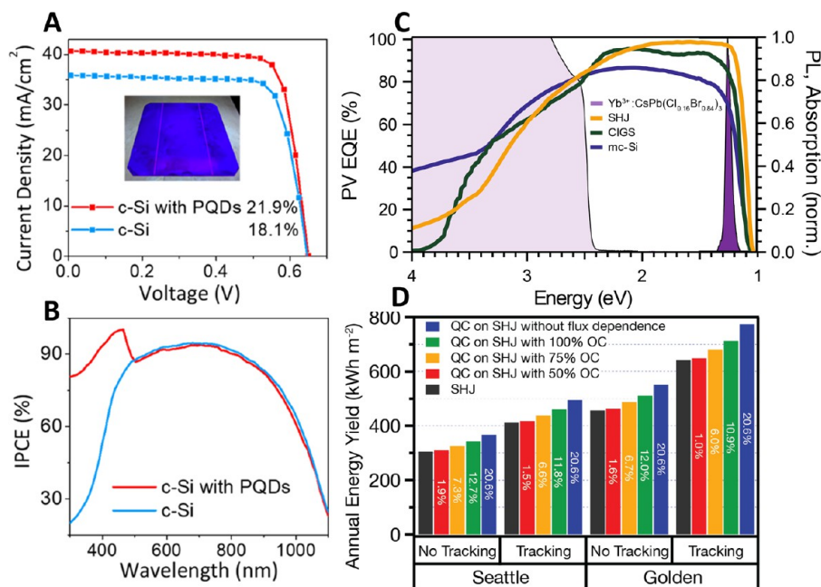
Figure 71. (A) J – V curves of a single-crystal silicon solar cell with and without a coating of Yb 3+ (6%)–Pr 3+ (4%)–Ce 3+ (3%)-tridoped CsPb(Cl 0.33 Br 0.67 ) 3 NCs, showing an increase in power-conversion efficiency from 18.1 to 21.9% upon addition of the NCs. (B) IPCE (EQE) curves of a single-crystal silicon solar cell with and without a coating of Yb 3+ (6%)–Pr 3+ (4%)–Ce 3+ (3%)-tridoped CsPb(Cl 0.33 Br 0.67 ) 3 NCs, showing enhancement at short wavelengths where the NCs absorb. (C) EQE characteristics of Si heterojunction (SHJ), CIGS, and multicrystalline Si photovoltaics and the absorption and near-infrared (~1.26 eV) emission of Yb 3+ :CsPb(Cl 0.16 Br 0.84 ) 3 quantum cutters, showing the excellent match of the quantum-cutter absorption and photoluminescence with the solar cell response curves, particularly for red-sensitive SHJ. (D) Areal annual energy production yield of a Yb 3+ :CsPb(Cl 1-x Br x ) 3 /SHJ QC/PV device with and without 2-axis tracking mechanisms and for different efficiencies of optical coupling, including the effects of flux-dependent PLQY. Relative percentage increases are labeled on each bar. Results are presented for two geographic locations in the United States: Seattle, WA, and Golden, CO. Panels A and B are reprinted from ref 661. Copyright 2019 American Chemical Society. Panels C and D are reprinted with permission from ref 657. Copyright 2019 Royal Society of Chemistry.
