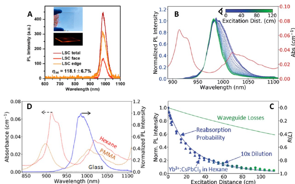
Figure 72. (A) Total (dark red), facial (light red), and edge (orange) emission spectra measured from a 5\text{ cm}^{-1} \times 5\text{ cm}^{-1} LSC made using \text{Yb}^{3+} -doped \text{CsPbCl}_3 NCs. The internal optical efficiency (edge-emitted photons/absorbed solar photons) of this device was measured to be 118 \pm 7\% . The top inset shows the high transparency of the LSC to visible light, and the bottom inset shows the LSC's edge emission under UV illumination, collected with a 570 nm long-pass filter. The PLQY of these NCs was measured to be 164 \pm 7\% prior to incorporation into the LSC. The optical density of this LSC at the perovskite absorption edge is 0.2. (B) Normalized PL spectra of \text{Yb}^{3+} : \text{CsPbCl}_3 NCs suspended in hexane with o.d. \sim 0.75 at 375 nm, obtained from a liquid 1D LSC experiment at various excitation distances relative to the edge-mounted photodetector (inset). The red curve shows the absorption spectrum of the hexane solvent. (C) Integrated normalized \text{Yb}^{3+} : \text{CsPbCl}_3 NC PL intensity plotted as a function of excitation distance away from the photodetector for NCs in hexane with o.d. \sim 0.75 (triangles) and o.d. \sim 0.075 (circles) at 375 nm. The blue trace is the reabsorption probability predicted from a model. The green line is the experimental performance limit of the 1D LSC waveguide itself. All PL data were collected with excitation at 375 nm, and all data were collected at room temperature. (D) Absorption spectrum of hexane (red), a representative PMMA sample (orange), and Schott optical-quality glass (black) overlaid with the normalized PL spectrum of \text{Yb}^{3+} : \text{CsPbCl}_3 NCs (blue). Panel A is adapted from ref 655. Copyright 2018 American Chemical Society. Panels B–D are adapted with permission from ref 656. Copyright 2019 Royal Society of Chemistry.
