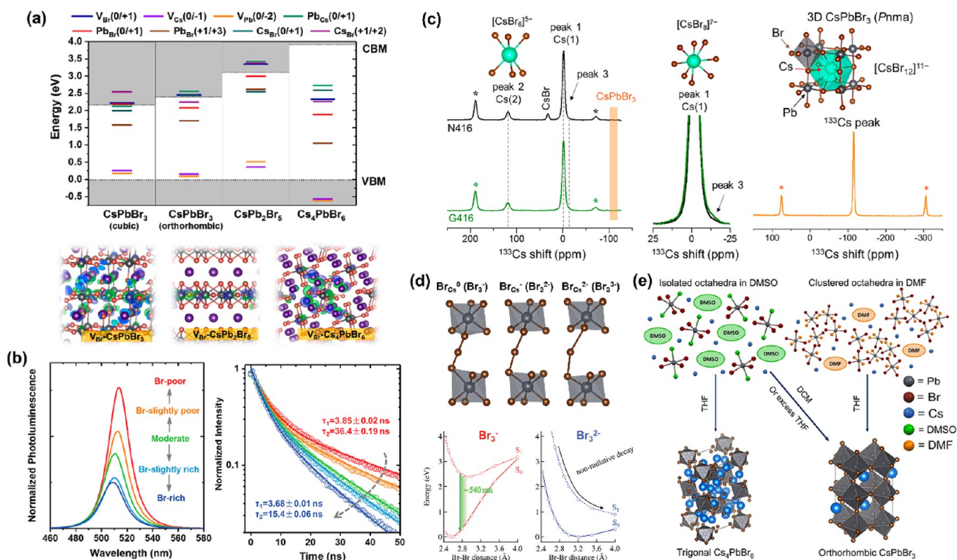
Figure 42. (a) Calculated defect charge transition levels and charge density distributions of V_{Br} defect states for CsPbBr 3 , CsPb 2 Br 5 , and Cs 4 PbBr 6 . (b) Normalized PL spectra and time-resolved PL spectra of Cs 4 PbBr 6 NCs under different growth conditions. Reproduced from ref 433. Copyright 2018 American Chemical Society. (c) 133 Cs MAS NMR spectra and corresponding magnified spectra (25 to −25 ppm) of non-emissive and green-emissive Cs 4 PbBr 6 obtained at 9.4 T and a spinning rate of 10 kHz at 300 K, together with 133 Cs MAS NMR spectra of CsPbBr 3 perovskite crystal. Reproduced from ref 434. Copyright 2020 American Chemical Society. (d) Local structure associated with point defect species in Cs 4 PbBr 6 and relative potential energy surfaces of ground state S 0 and first excited state S 1 as a function of the Br–Br distance for Br 3 - and Br 3 2- . Reproduced with permission from ref 435. Copyright 2019 Royal Society of Chemistry. (e) Schematic diagram of the effect of the solvodynamic size and solvent–antisolvent pair on the formed CsPbBr 3 and Cs 4 PbBr 6 phases. Reproduced under a Creative Commons CC-BY-NC-ND license from ref 436. Copyright 2019 American Chemical Society.
