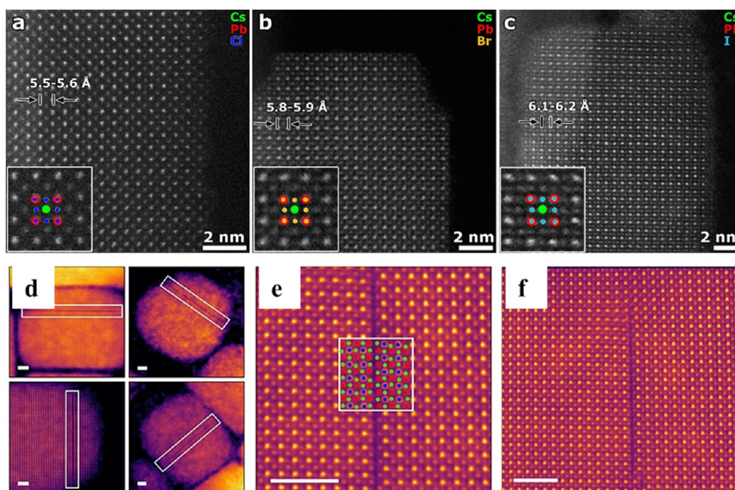
Figure 79. High-resolution HAADF-STEM images of a (a) CsPbCl 3 , (b) CsPbBr 3 , and (c) CsPbI 3 perovskite nanowire. The different atomic columns are identified using the intensity–atomic number relation in HAADF-STEM imaging. Reproduced with permission from ref 22. Copyright 2016 John Wiley & Sons, Inc. (d) Overview HAADF-STEM images showing the presence of Ruddlesden–Popper planar defects (highlighted as rectangular boxes) in several CsPbBr 3 NCs. (e) Atomic-resolution HAADF-STEM image of a Ruddlesden–Popper planar defect with an overlaid atomic model (blue, Pb; red, Cs; green, Br). (f) Atomic-resolution HAADF-STEM image of a Ruddlesden–Popper planar defect extending only a few unit cells. The scale bars correspond to 3 nm. Reproduced from ref 707. Copyright 2018 American Chemical Society.
