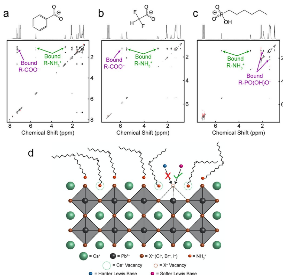
Figure 31. 1 H NOESY NMR spectra of CsPbBr 3 NC samples exchanged to ligand pairs of oleylammonium and (a) benzoate, (b) difluoroacetate, and (c) hexylphosphonate. All ligand pairs feature negative (black) NOE signals rather than positive (red) NOE signals, thereby corroborating their interaction with the NC surface. (d) Schematic representation of a cesium- and halide-deficient surface terminated by CsX facets, consistent with experimental results. Reproduced from ref 194. Copyright 2018 American Chemical Society.
