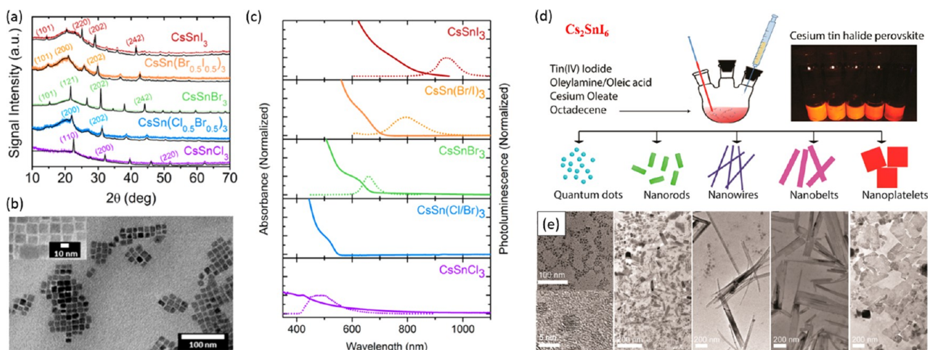
Figure 51. (a) XRD pattern of CsSnX 3 (X = Cl, Cl 0.5 Br 0.5 , Br, Br 0.5 I 0.5 , I) perovskite NCs synthesized by the hot-injection method. (b) TEM images and (c) UV-vis-NIR absorbance and PL spectra of CsSnX 3 NCs of different halide compositions. (d) Schematic illustration of the synthesis of Cs 2 SnI 6 perovskite NCs by the hot-injection approach (left panel) and photograph of the prepared colloidal solutions of Cs 2 SnI 6 NCs under UV light (right panel). (e) Corresponding TEM images of the Cs 2 SnI 6 NCs of different morphologies. Panels a–c are reprinted under a Creative Commons CC-BY License from ref 515. Copyright 2016 American Chemical Society. Further permissions related to the material excerpted should be directed to the ACS. Panels d and e are adapted from ref 522. Copyright 2016 American Chemical Society.
