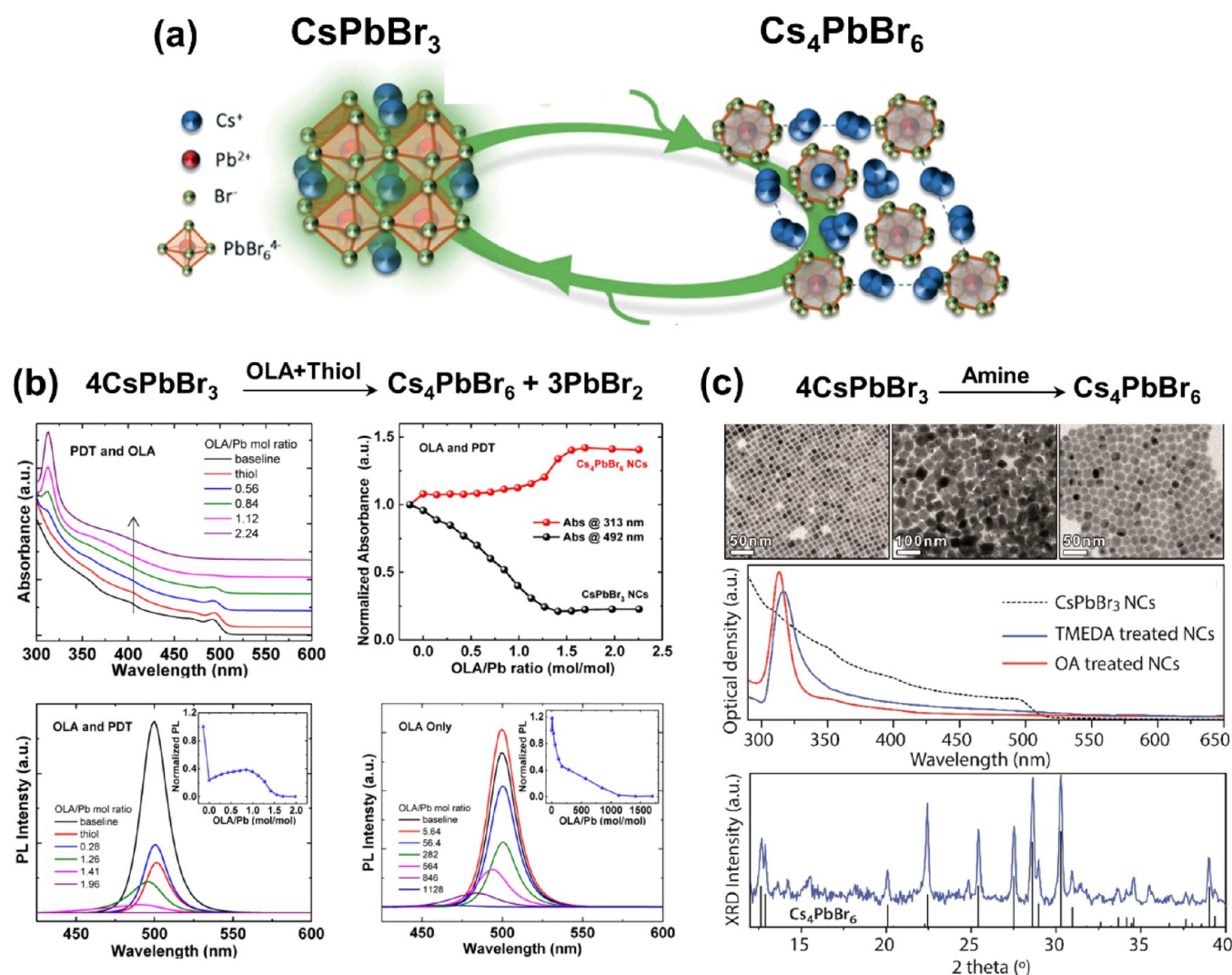
Figure 37. (a) Schematic illustration of the structural transformation between \text{CsPbBr}_3 and \text{Cs}_4\text{PbBr}_6 NCs. Reproduced with permission from ref 420. Copyright 2018 Royal Society of Chemistry. (b) Absorbance spectra, normalized absorbance at two spectral features, and PL spectra of \text{CsPbBr}_3 NCs solutions before and after adding different amount of oleylamine with and without PDT. Reproduced from ref 421. Copyright 2017 American Chemical Society. (c) TEM micrographs, absorption spectra, and XRD patterns of \text{CsPbBr}_3 NCs before and after the treatment with either tetramethylethylenediamine (TMEDA) or OA. Reproduced from ref 422. Copyright 2017 American Chemical Society.
