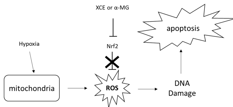
Figure 4. During hypoxia, mitochondrial reactive oxygen species (ROS) are induced exponentially. This could lead to DNA damage, which could induce apoptosis. Nrf2 is usually activated during this event to trigger an event that neutralizes ROS. Inhibition of NRF2 by XCE or α-MG disrupts ROS neutralization, promoting cell death by apoptosis.
