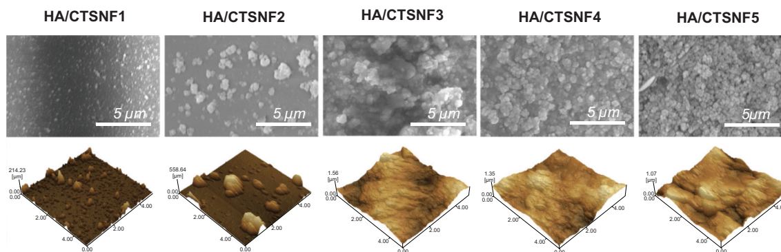
Figure S2 SEM and AFM images of HA/CTS NF substrates with different HA/CTS ratios.
