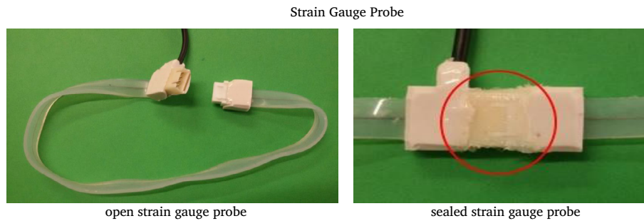
Figure 1. (A) The strain gauge plethysmography probe. (B) Sealed probe. Note the liquid metal embedded in a silicon band (arrow).
