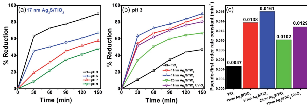
Fig. 3 (a) Photo-reduction of Cr(vi) at different pH values using 17 nm \text{Ag}_2\text{S}/\text{TiO}_2 nanofibers, (b) photo-reduction using variable sized \text{Ag}_2\text{S}/\text{TiO}_2 nanofibers at pH 3 compared to the pristine \text{TiO}_2 nanofibers, and (c) the corresponding pseudo-first order rate constants.
