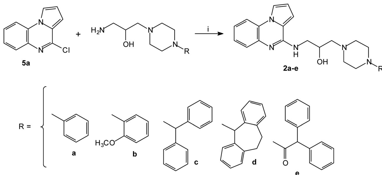
Scheme 3 Synthesis of piperazinylalcohol-pyrrolo[1,2- a ]quinoxalines 2a–e ; reagents and conditions: (i) K 2 CO 3 , DMF, 120 °C.
