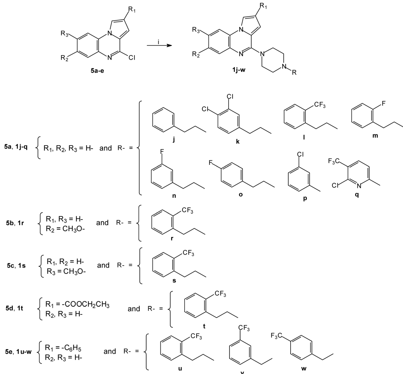
Scheme 2 Synthesis of 4-(4-substituted-piperazinyl)-4-phenylpyrrolo[1,2-a]quinoxalines 1j-w ; reagents and conditions: (i) R -piperazine, Pd 2 (dba) 3 , BINAP, t -BuONa, toluene, 100 °C.
