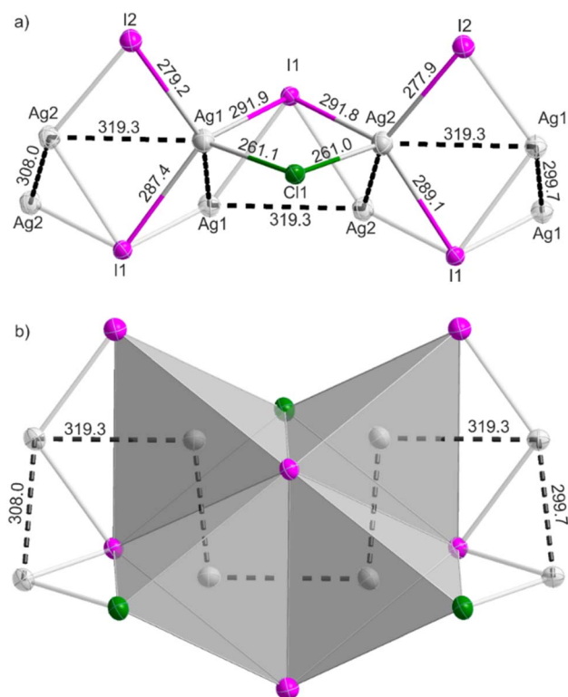
Fig. 4 \infty [AgI_{2/4}I_{1/2}Cl_{1/2}]^- chain with d^{10} – d^{10} interaction in [EMIm][AgI_2Cl] ( 6 ).
