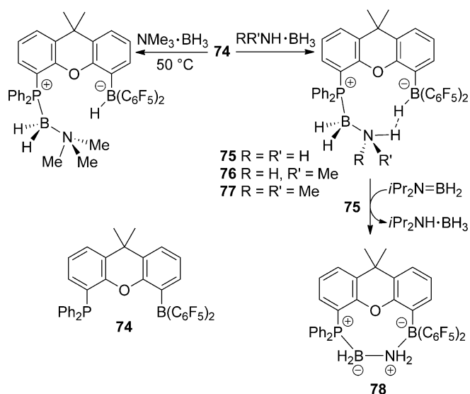
Scheme 37. Stoichiometric reactions of 74 with amine-boranes.
