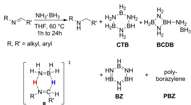
Scheme 6. Dihydrogen transfer from AB to imines.
