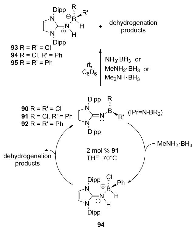
Scheme 44. Reactivity of N-heterocyclic iminoboranes towards different amine-boranes.
