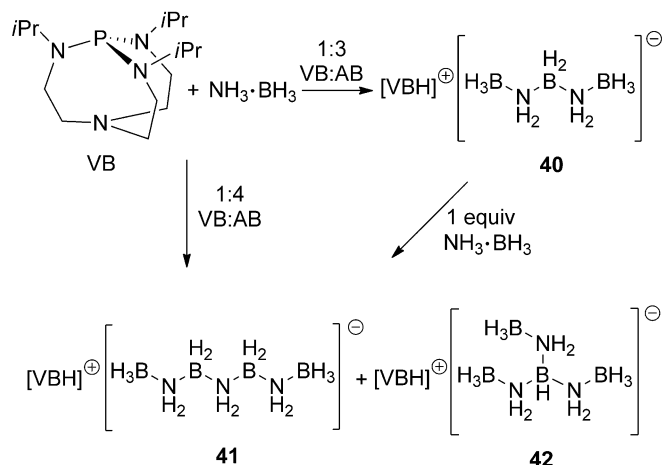
Scheme 23. Formation and isolation of intermediates in the base-promoted polymerization of AB.
