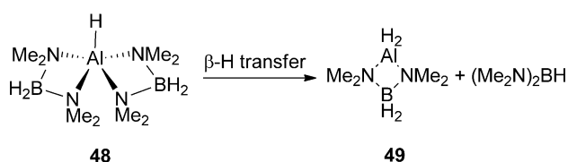
Scheme 26. \beta -hydride transfer to form 49 .
