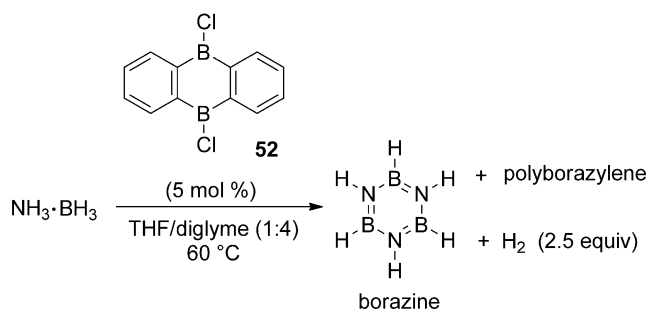
Scheme 28. Catalytic dehydrogenation of \text{NH}_3\cdot\text{BH}_3 by 52 .
