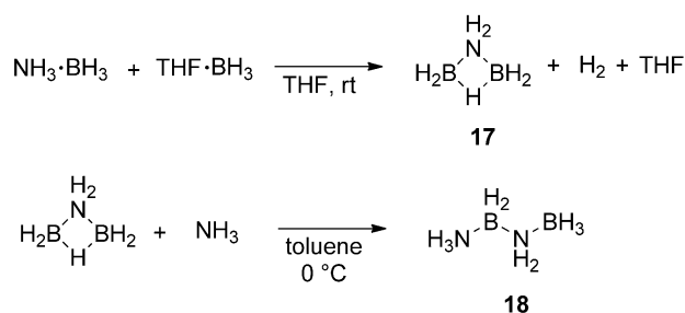
Scheme 12. Formation and reactivity of aminodiborane 17 .
