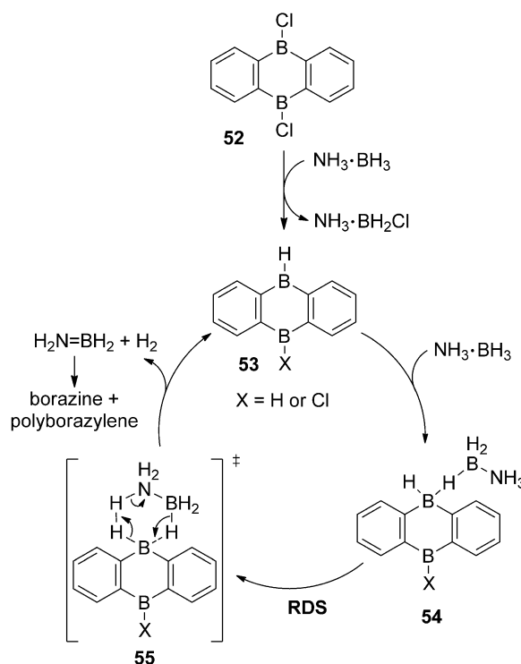
Scheme 29. Mechanism of AB dehydrogenation by 53 .
