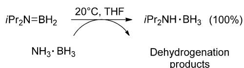
Scheme 1. Reaction of i\text{Pr}_2\text{N}=\text{BH}_2 with \text{NH}_3\cdot\text{BH}_3 .
