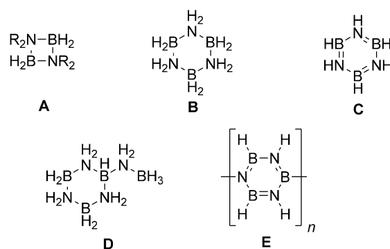
Figure 1. B–N-containing products.
