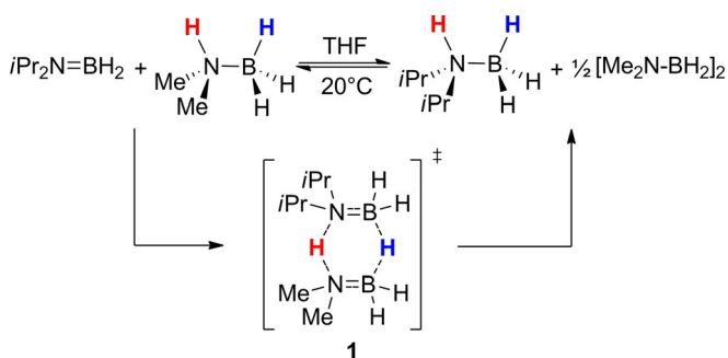
Scheme 2. Equilibrium formation during the reaction of i\text{Pr}_2\text{N}=\text{BH}_2 with \text{Me}_2\text{NH}\cdot\text{BH}_3 .
