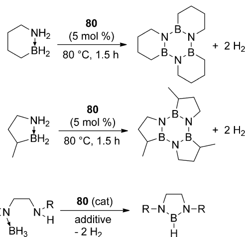
Scheme 39. Catalytic dehydrogenation of cyclic amine–boranes and diamine–boranes with 80 .
