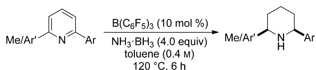
Scheme 43. FLP-catalyzed transfer hydrogenation of pyridines.
