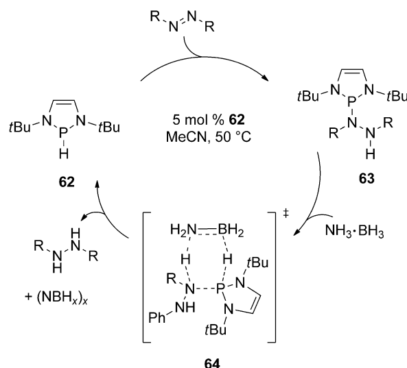
Scheme 33. Proposed catalytic cycle for azobenzene hydrogenation catalyzed by 62 .
