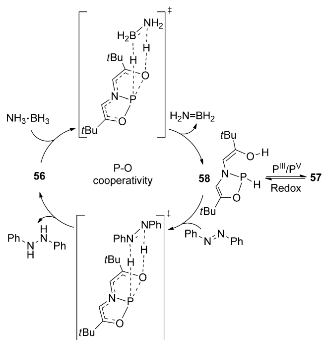
Scheme 31. Calculated catalytic cycle for azobenzene transfer hydrogenation.
