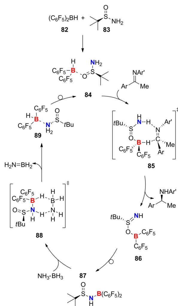
Scheme 41. FLP-catalyzed asymmetric transfer hydrogenation of imines.
