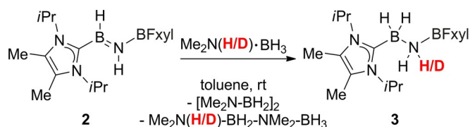
Scheme 3. Dihydrogen abstraction from \text{Me}_2\text{NH}\cdot\text{BH}_3 with 2 (F xyl = 3,5-(F 3 C) 2 C 6 H 3 ).
