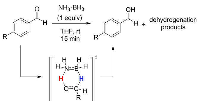
Scheme 9. Chen's proposed mechanism for hydrogen transfer of AB to aldehydes.
