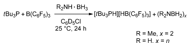
Scheme 18. Dehydrogenation of amine–boranes utilizing PtBu_3/B(C_6F_5)_3 .
