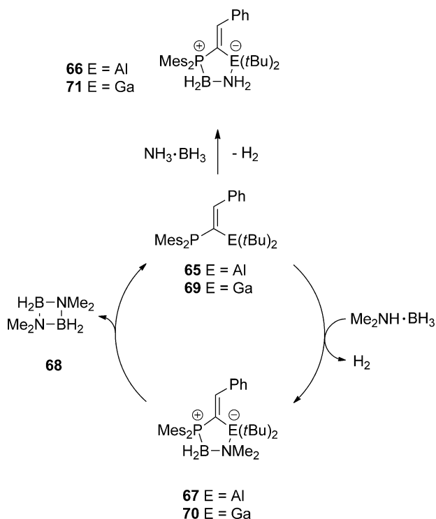
Scheme 34. Amine-borane dehydrogenation by a P/E (E = Al, Ga) FLP.
