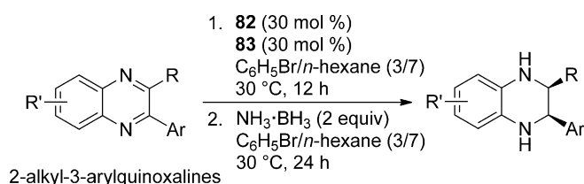
Scheme 41. FLP-catalyzed asymmetric transfer hydrogenation of imines.
