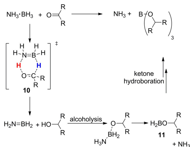
Scheme 8. Proposed mechanism by Zhou and Fan for alkyl borate formation.
