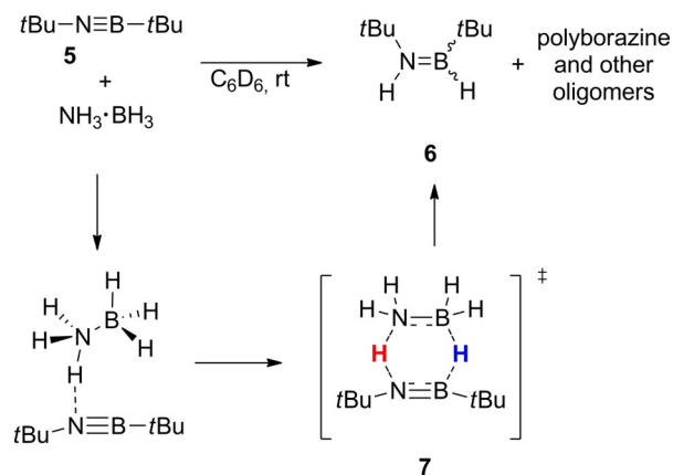
Scheme 5. Computed mechanism for dihydrogen transfer from AB to iminoboranes.
