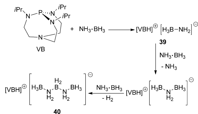
Scheme 22. Anionic polymerization of AB dehydrogenation initiated by a Brønsted base.
