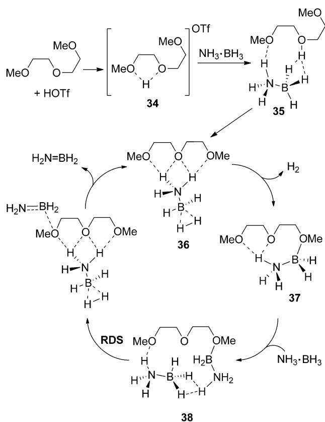
Scheme 21. Calculated mechanism for ammonia-borane dehydrogenation using triflic acid in diglyme.
