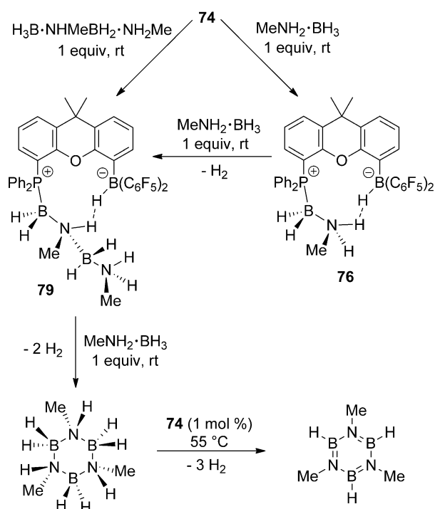
Scheme 38. Stoichiometric and catalytic reactions of 74 with methylamine–boranes.
