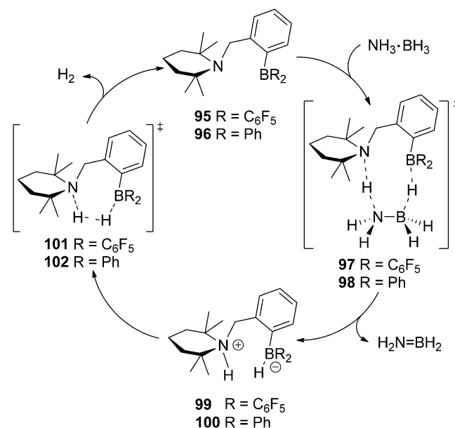
Scheme 45. Calculated mechanism for ammonia-borane dehydrogenation.
