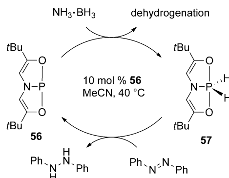
Scheme 30. Proposed catalytic cycle for azobenzene hydrogenation.
