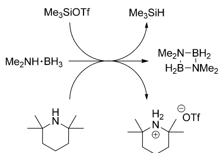
Scheme 19. Dehydrogenation of amine-boranes mediated by \text{Me}_3\text{SiOTf}/\text{TMP} .
