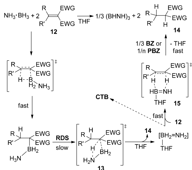
Scheme 10. Reduction of C=C double bonds through hydrogen transfer of ammonia-borane.
