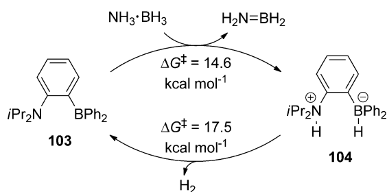
Scheme 46. Energy barriers for 103 for ammonia–borane dehydrogenation.
