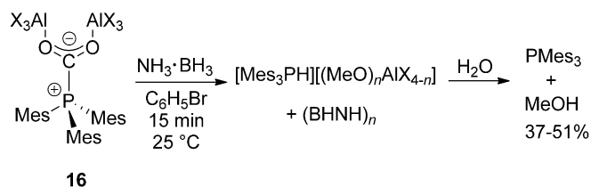
Scheme 11. Transition-metal-free conversion of \text{CO}_2 to methanol.
