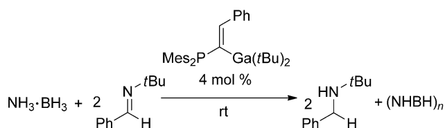
Scheme 35. FLP 69 as catalyst for imine hydrogenation.
