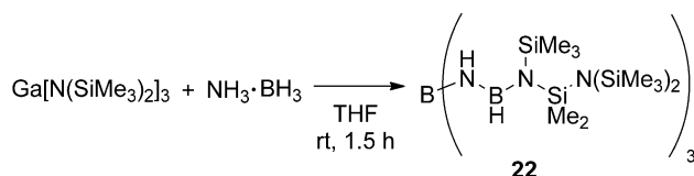
Scheme 14. Reactivity of a gallium(III)-based complex with NH_3 \cdot BH_3 .
