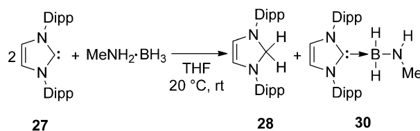
Scheme 17. 2:1 reaction of an NHC with MeNH_2 \cdot BH_3 .
