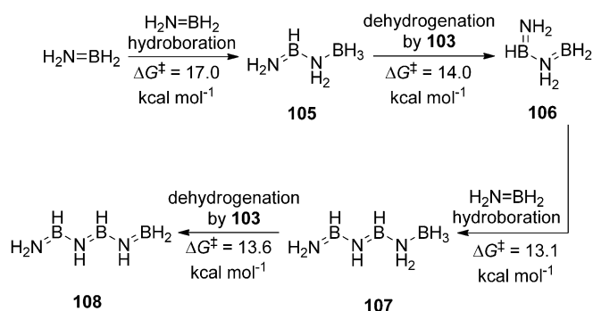
Scheme 47. Oligomerization of aminoborane monomers assisted by 103 .
