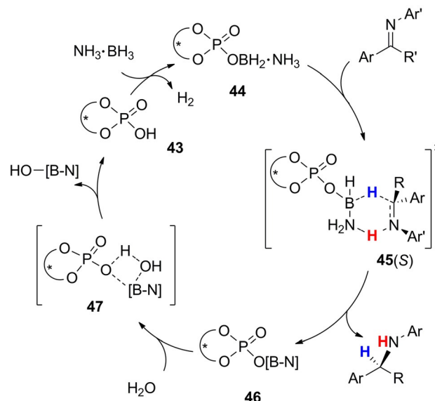
Scheme 25. Mechanism for transfer hydrogenation by 43 (shown schematically here).
