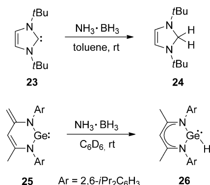
Scheme 15. The reaction of an N-heterocyclic carbene and germylene with AB.
