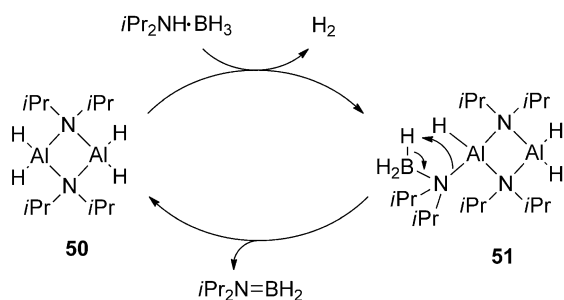
Scheme 27. Mechanism for i\text{Pr}_2\text{NH}\cdot\text{BH}_3 dehydrogenation by 50 .
