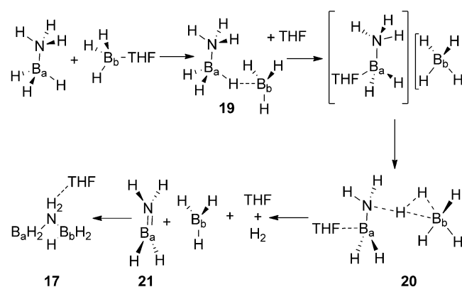
Scheme 13. Proposed mechanism for the formation of aminodiborane from \text{NH}_3\text{·BH}_3 and \text{THF·BH}_3 .
