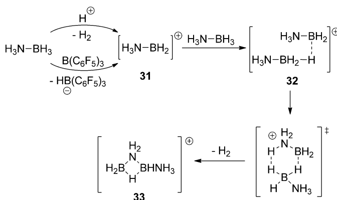
Scheme 20. Initiation step of AB dehydrogenation by Brønsted and Lewis acids.
