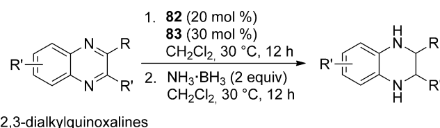
Scheme 42. FLP-catalyzed reduction reactions of 2,3-disubstituted quinoxalines.
