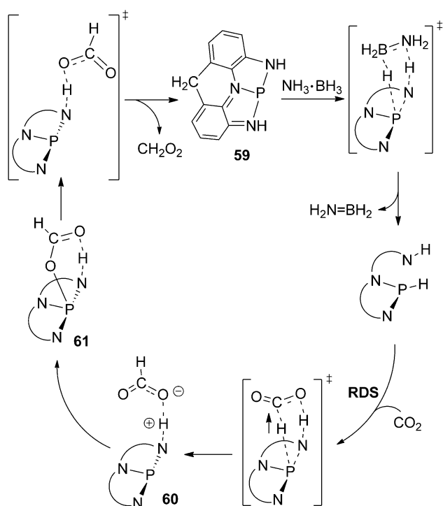
Scheme 32. Catalytic transfer hydrogenation by a pincer-type phosphorus compound.
