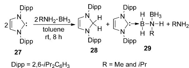
Scheme 16. Dehydrogenation of RNH_2 \cdot BH_3 by an NHC.
