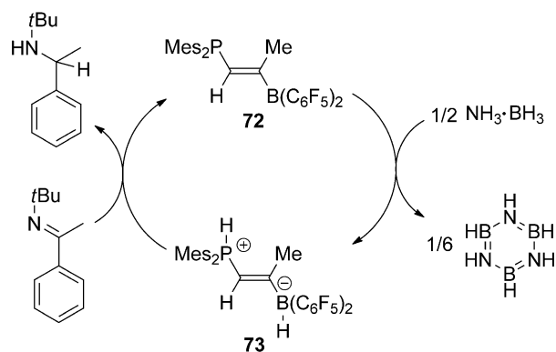
Scheme 36. Phosphinoborane-catalyzed transfer hydrogenation of imines.
