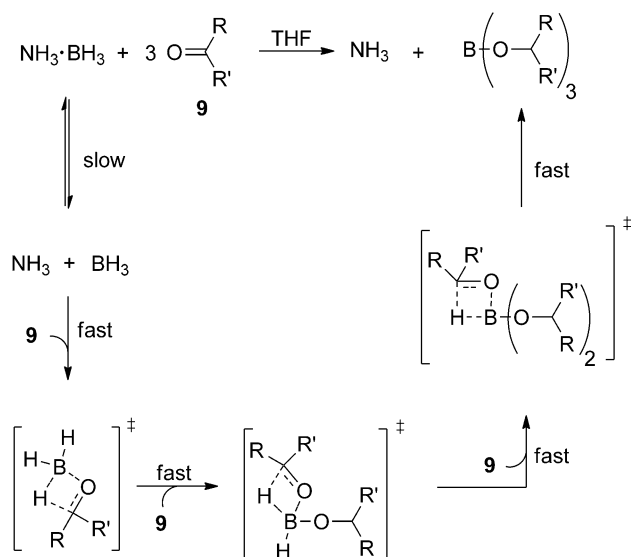
Scheme 7. Hydroboration of ketones and aldehydes.
