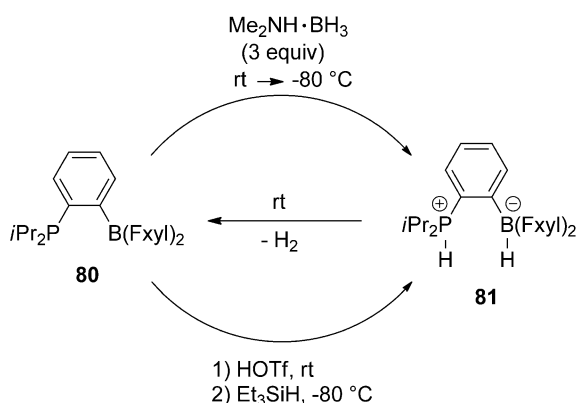
Scheme 40. Stepwise and catalytic generation of phosphonium–borate 81 .
