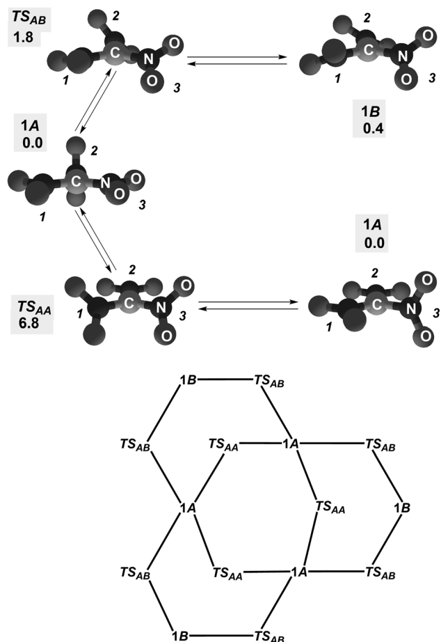
Fig. 3 Interconversion of conformers 1A and 1B . Top: interconversion in the pair 1A and 1B and interconversion in the pair of two degenerate conformers 1A . Bold numbers with gray background indicate calculated relative free energies ( \text{kcal mol}^{-1} ) for these structures, and numbers in bold italics are formal labels of \text{NO}_2 groups. For clarity, the central atom and atoms of one \text{NO}_2 group are supplied with related chemical element symbols. Bottom: the representative graph of conformational pathways for anion 1 (interconversion of three degenerate conformers 1A and three degenerate conformers 1B of axial chirality R_a ).
