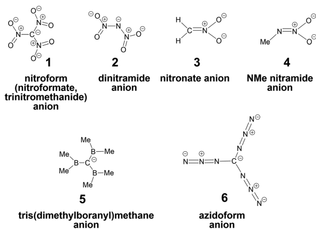
Fig. 1 Chemical structure of anions 1–6 shown in a plain notation of localized bonds. This formal view is very far from reflecting the chemical bonding in 1–6 .
