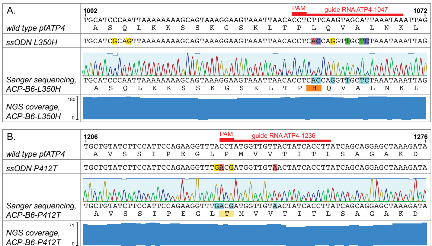
Fig 2. Sequencing results. Sanger and NGS sequencing coverage of targeted CRISPR mutations at the pfatp4 locus for ACP-B6-L350H and ACP-B6-P412T with clonal wild type parent strain ACP-B6. Red bars delineate the respective 20 nt guide RNA target sites and PAM sites required for each edit. NGS coverage at each location is indicated by blue columns. (a) Sequencing data of targeted locus 1002–1072 in pfatp4 from strain ACP-B6-L350H showing SJ733 resistance-conferring SNPs in L350 and four other synonymous mutations introduced by CRISPR. Sequences of wild type pfatp4 and repair template ssODN L350H are shown in alignment. The two silent mutations in ssODN L350H located 39 and 42 nt away were not incorporated into ACP-B6-L350H. (b) Sequencing data of targeted locus 1206–1276 in pfatp4 from strain ACP-B6-P412T showing the SJ733 resistance-conferring SNP and silent mutations introduced by CRISPR. Sequences of wild type pfatp4 and repair template ssODN P412T are shown in alignment.
