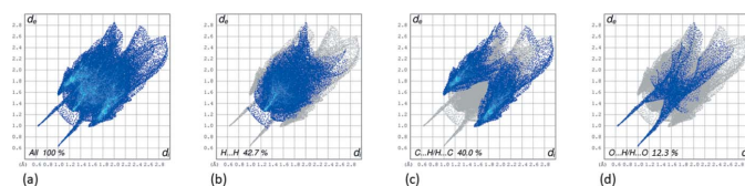
Figure 5 (a) The two-dimensional fingerprint plots of the title compound, and delineated into (b) H...H (42.7%), (c) C...H/H...C (40.0%) and (d) O...H/H...O (12.3%) contacts.
