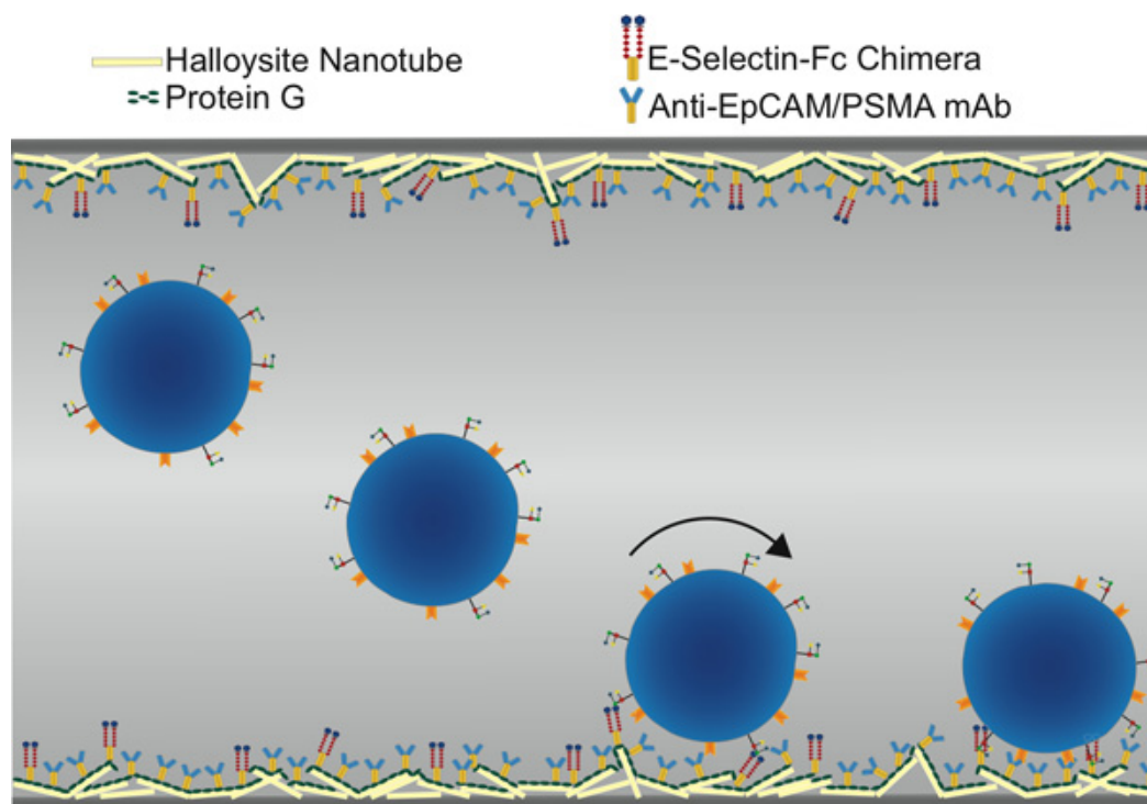
Figure 1. Schematic of functionalized microtube for CTC isolation, showing selectin-mediated rolling followed by antibody-mediated static adhesion.
