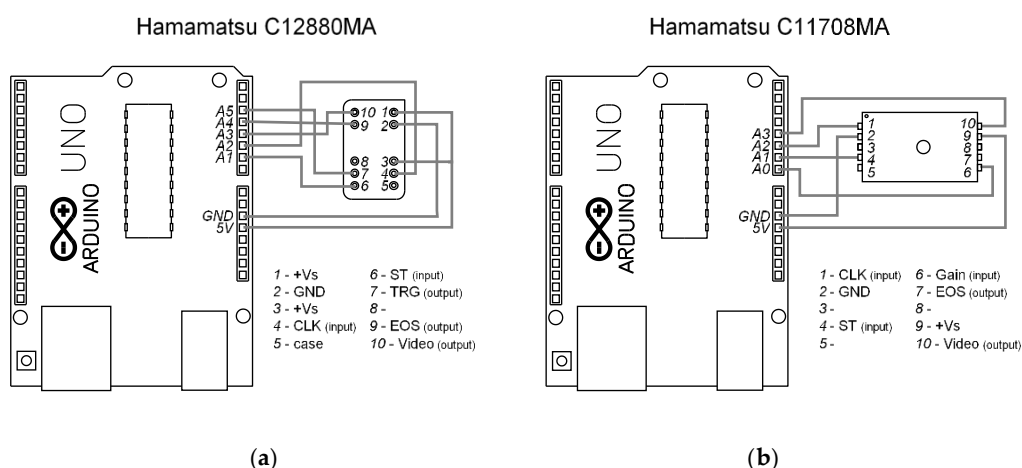
Figure 5. Connection diagram of Hamamatsu C12880MA (a) and C11708MA (b) micro-spectrometers to the Arduino UNO microcontroller.
