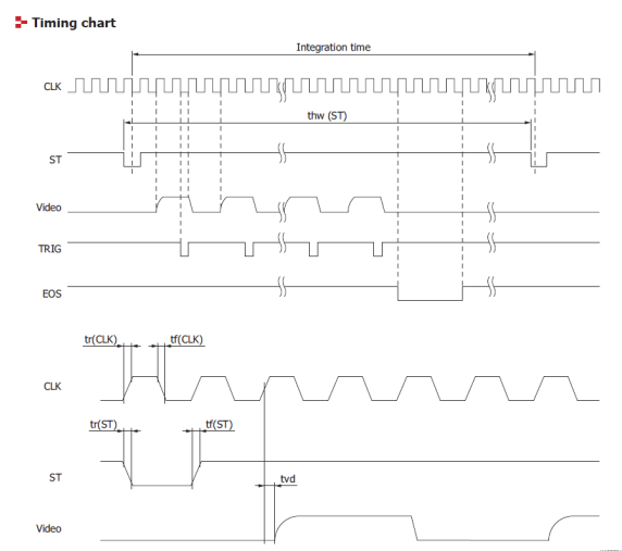
Figure A1. Timing chart for signal input and output for micro-spectrometer Hamamatsu C12880MA (source: https://www.hamamatsu.com/resources/pdf/ssd/c10988ma-01_etc_kacc1169e.pdf ).
