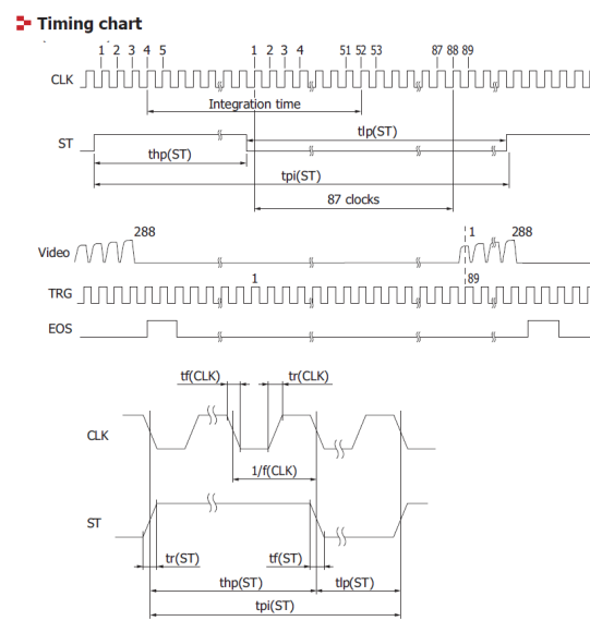
Figure A2. Timing chart for signal input and output for micro-spectrometer Hamamatsu C12880MA (source: https://www.hamamatsu.com/resources/pdf/ssd/c12880ma_kacc1226e.pdf ).
