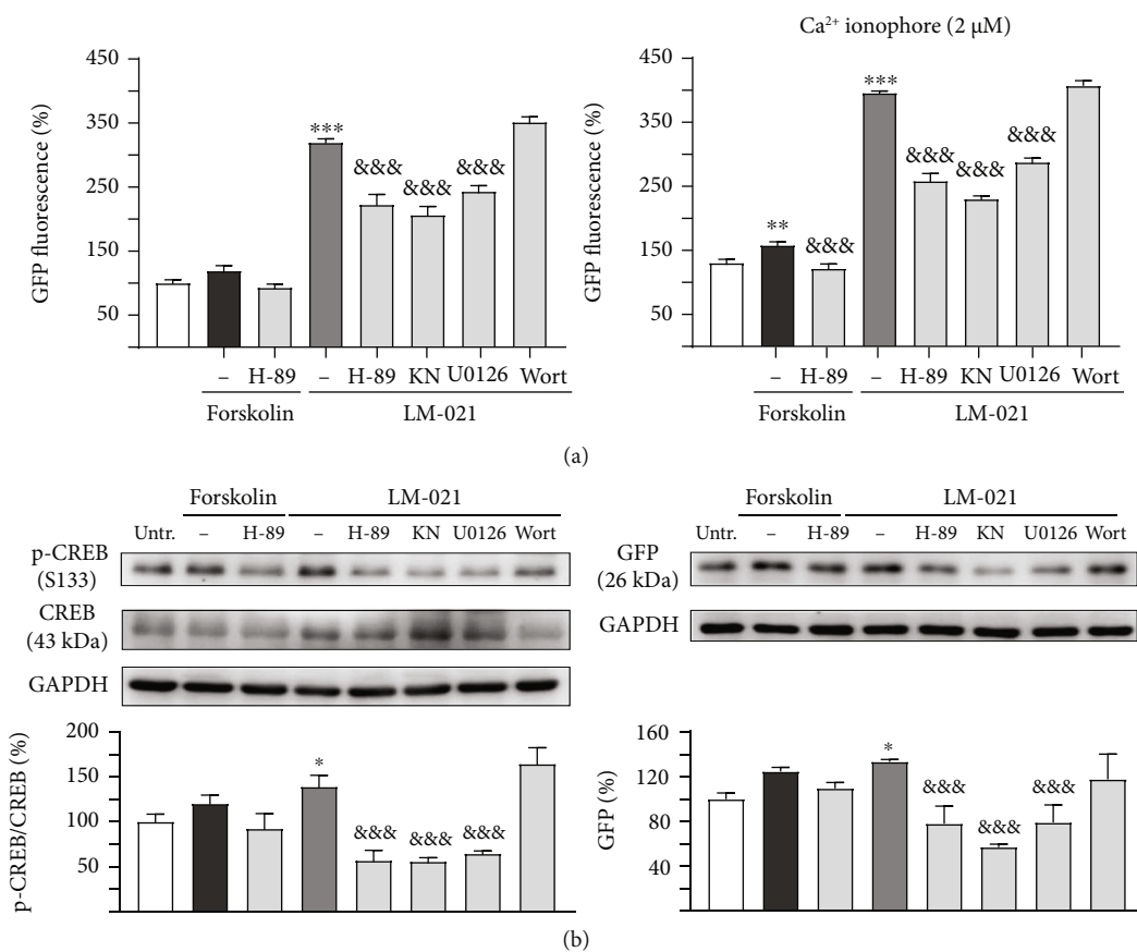
FIGURE 5: LM-021-mediated kinase activation in CRE-GFP reporter cells. (a) Fluorescence analysis of CRE reporter cells without and with kinase inhibitor, Ca 2+ ionophore, and/or forskolin or LM-021 treatment. GFP fluorescence was assessed by flow cytometry ( n = 3 ). To normalize, the GFP fluorescence level in untreated cells was set as 100%. (b) p-CREB and GFP levels analysed by immunoblot using GAPDH as a loading control ( n = 3 ). To normalize, the protein expression level in untreated cells was set as 100%. p values: compound treated vs. untreated cells ( *p < 0.05 , **p < 0.01 , and ***p < 0.001 ), or kinase inhibitor-treated vs. untreated cells ( \&\&\& : p < 0.001 ) (one-way ANOVA with a post hoc Tukey test).
