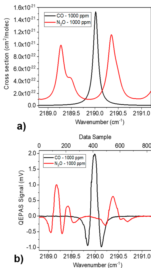
Figure 2. (a) HITRAN simulation of absorption cross section spectrum and (b) QEPAS scan of 1000 ppm of CO in \text{N}_2 (black curve) and 1000 ppm of \text{N}_2\text{O} in \text{N}_2 (red curve).
