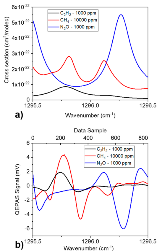
Figure 5. (a) HITRAN simulation of the absorption cross section spectrum and (b) QEPAS scan of 1000 ppm of C 2 H 2 in N 2 (black curve), 10 000 ppm of CH 4 in N 2 (red curve), and 1000 ppm of N 2 O in N 2 (blue curve).
