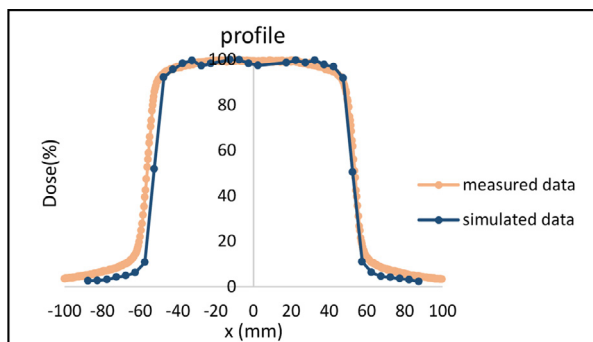
Figure 2: Profile curves calculated by Monte Carlo simulation and measured by the ionizing chamber, field size 10×10 cm 2 .
