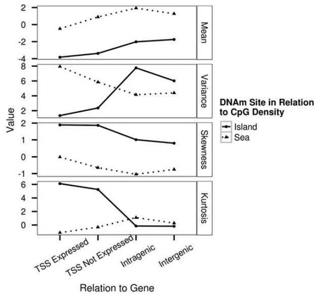
Figure 4. Moments of the distributions of mean site-specific DNAm level for eight contextual groups.
