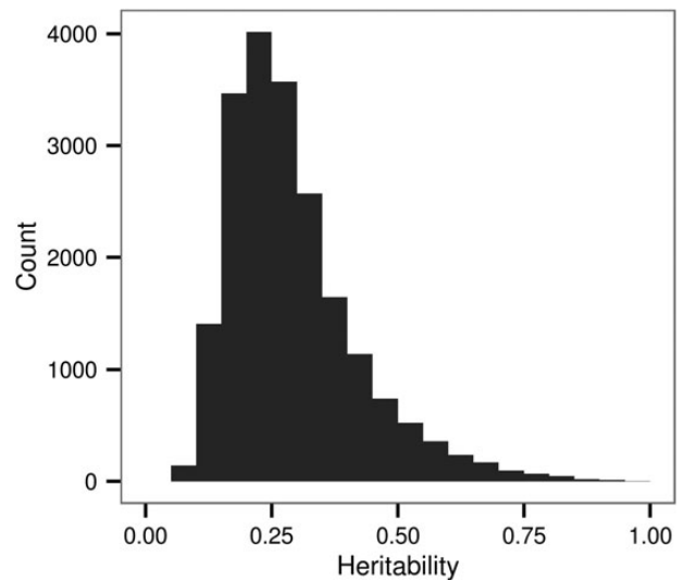
Figure 6. Distribution of the estimated heritability for DNAm sites significantly associated with local genetic variation. Each bar represents a range of 0.05.
