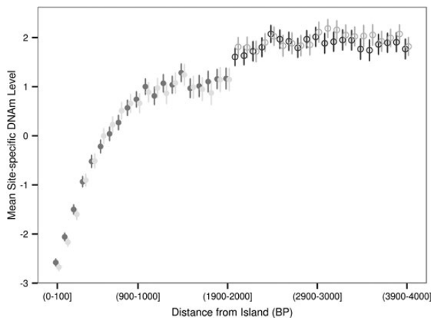
Figure 2. Mean site-specific DNAm level as a function of distance from the edge of the island. The 4000 BP region upstream (North) and downstream (South) of islands was divided into bins of 100 BP. The average of the mean site-specific DNAm levels for DNAm sites residing within each bin is shown as a circle enclosed by a line indicating \pm 2 standard error of the mean estimate. A shore is up to 2000 BP from an island and a shelf is between 2000 and 4000BP from an island.
