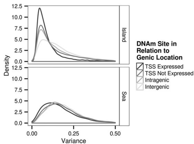
Figure 5. Distribution of the variance of each DNAm site used in analysis ( n = 196080 ).
