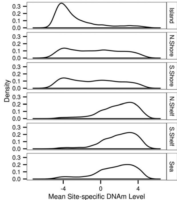
Figure 1. Distribution of mean site-specific DNAm level with respect to CpG density. Methylation levels were measured on the M -value scale where a DNAm level of 0 can be interpreted as a 50% methylation level, a DNAm level of <0 and a DNAm level of >0 indicate < and >50% methylation, respectively. The majority of DNAm sites in islands exhibited a low-average methylation level, which was in contrast to the majority of DNAm sites in low-density CG regions (sea) being on average highly methylated.
