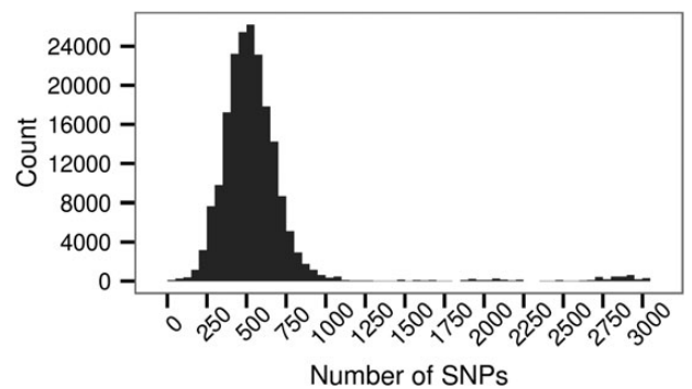
Figure 7. The number of SNPs \pm 1 MB surrounding a DNAm site.
