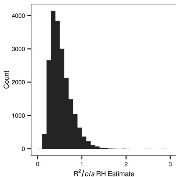
Figure 10. Proportion of the regional heritability that can be explained by the top SNP association. The variance explained by a SNP ( R^2 ) divided by the regional heritability estimate for DNAm sites with a regional heritability estimate significant at P < 0.05 . Only the most significant SNP within the local region was considered. In 4.2% of cases the SNP explained more variance in the DNAm level than did the region.
