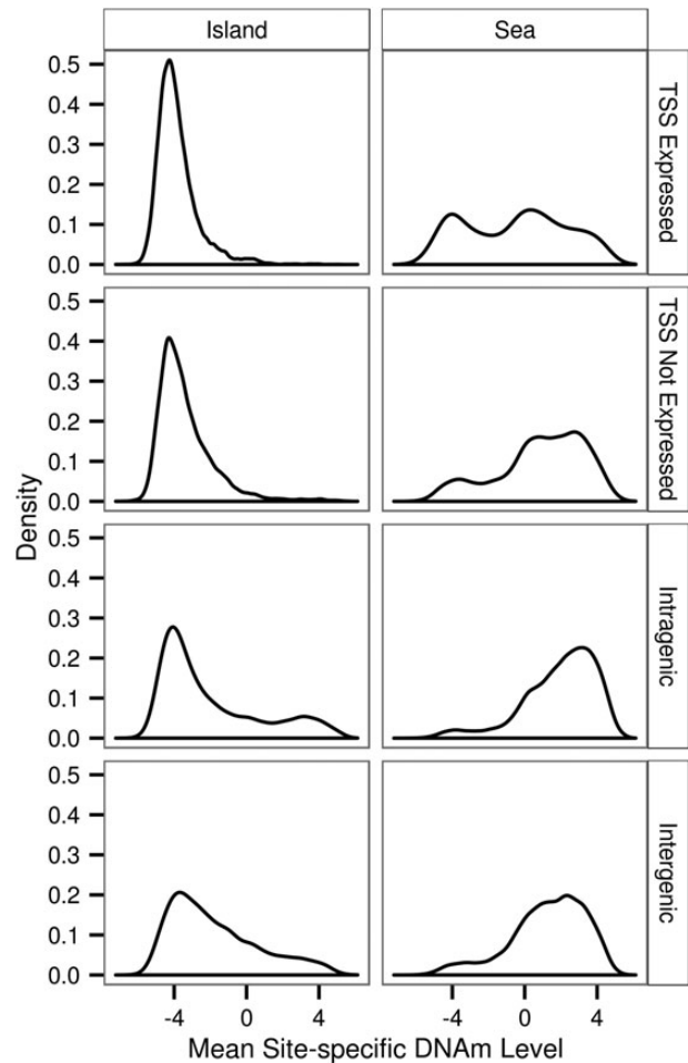
Figure 3. Distribution of mean site-specific DNAm level for eight contextual groups.
