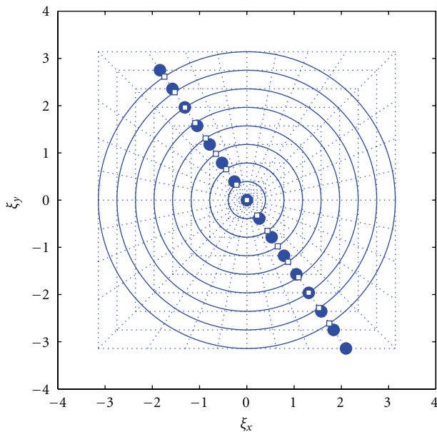
FIGURE 4: Circle the squares interpolation stage. Circles denote the known pseudo-Polar grid points while the squares are the destination equiangular spaced rays. (This figure first appeared in [33]).
