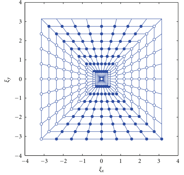
FIGURE 2: Basically vertical subnet (filled circles) and basically horizontal subnet (hollow circles) comprising the pseudo-Polar grid formed by the intersection of 8 concentric squares and 16 slope-equispaced rays. (This figure first appeared in [33]).
