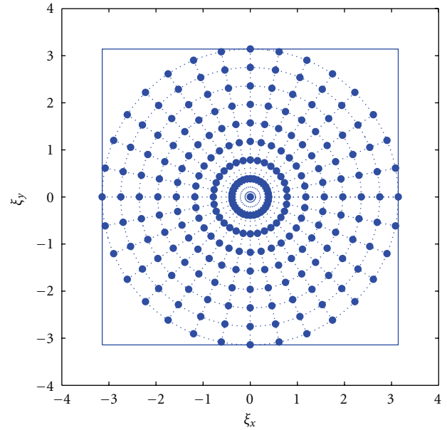
FIGURE 5: Final Polar grid points after both interpolation processes have been applied. (This figure first appeared in [33]).
