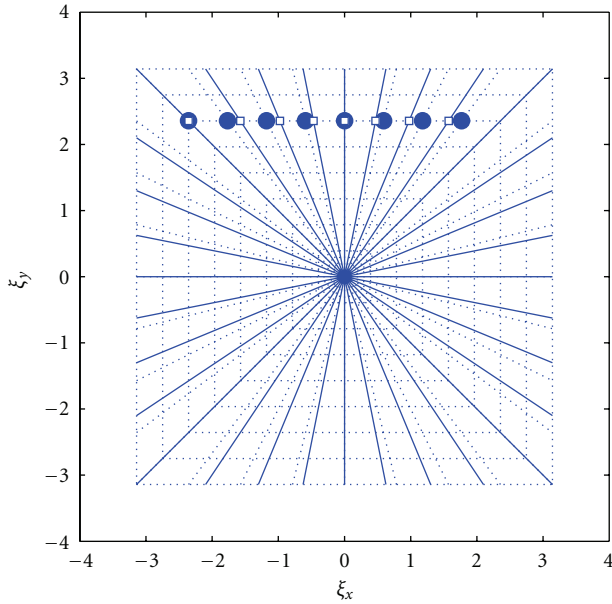
FIGURE 3: Rotate the rays interpolation stage. Circles denote the known pseudo-Polar grid points while the squares are the destination equiangular spaced rays. (This figure first appeared in [33]).
