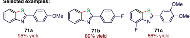
Scheme 25 C-H thiolation.
