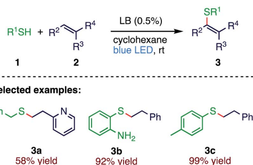
Scheme 1 Photocatalyzed thiol–ene reaction.
