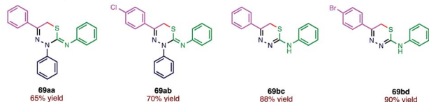
Scheme 24 Synthesis of 1,3,4-thiadiazines.
