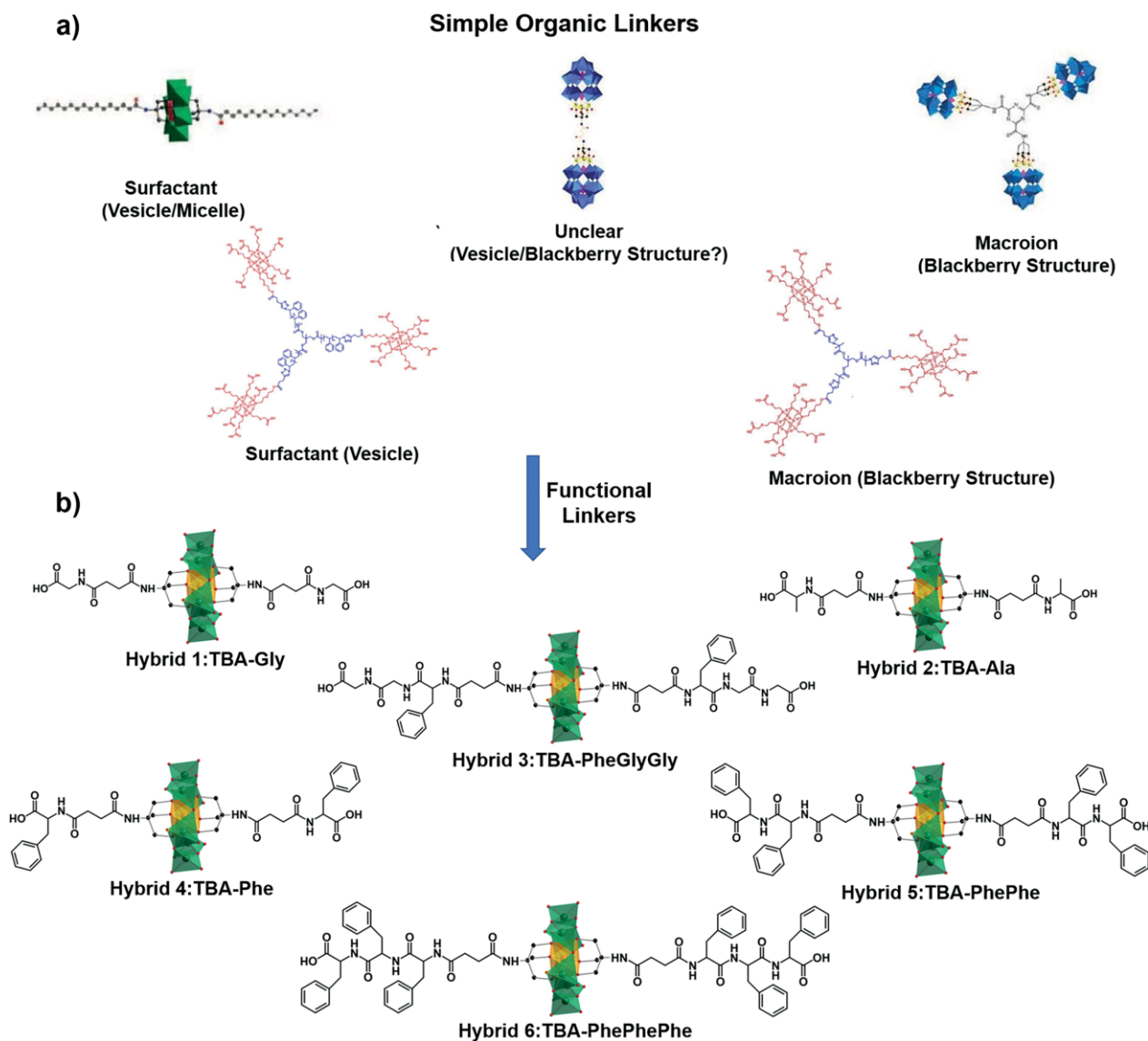
Figure 1. a) Molecular structures of hybrids with simple organic linkers. b) Molecular structures of six POM-peptide hybrid clusters with the functional tails.
