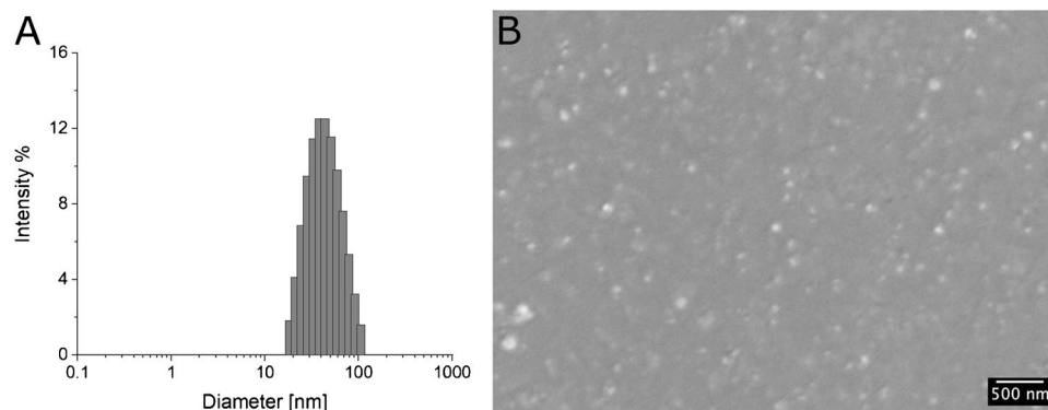
Fig. 1 BioMIP size distribution obtained by DLS (A) and micrograph obtained by SEM after freeze-dried on top of a silicon slide (B)
